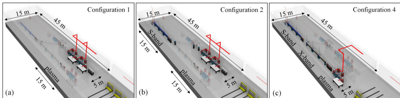
Figure 3: The preliminary layout of the EUPRAXIA accelerator tunnel is shown [41]. All RF and laser infrastructure is being supplied from the level above (not shown). Undulators (yellow) are shown in the bottom right corners. (a) Configuration 1: LWFA with internal injection. Two plasma stages are included which are supplied with two laser beams (red). (b) Configuration 2: LWFA with external injection from an RF accelerator. The RF gun and three S-band structures are shown in front of a dogleg which transports the electrons to the two plasma stages. (c) Configuration 4: PWFA. Using the same infrastructure of RF gun and S-band structure, the PWFA case uses additional X-band structures to accelerate the beam to several hundred MeV before using it inside a single plasma accelerator stage.
