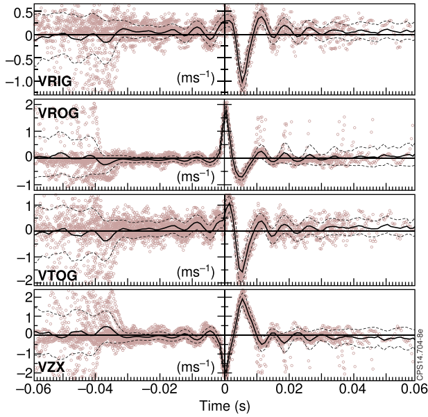
FIG. 10. Plasma edge velocity, offset so that they are zero at the ELM time ( t = 0 ). From top to bottom: the velocity of plasma motion at the inner gap (VRIG), outer gap (VROG), plasma top (VTOG), and plasma's X-point (VZX). The absolute magnitude of the velocity depends on the numerical method by which the velocity is estimated, that requires the signal to be smoothed, but is in metres per second (vertical axis) with the horizontal (time) axis being in seconds. The velocities are slightly underestimated here, but the resulting signal shape is approximately independent of the smoothing procedure. Circles are from a typical pulse (83 794), the solid line is an average across the pulse set, and the dashed lines are the average \pm the standard deviation.
