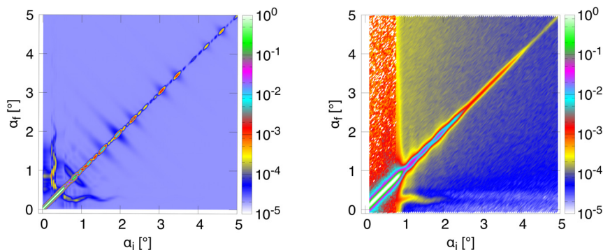
Fig. 6. Simulated and experimental off-specular scattering of the resonator with surface roughness (rms = 0.1 nm, correlation length \xi = 1 \mu\text{m} , and the hurst parameter = 0.8 [33,34], \lambda = 6 \text{ \AA} , constant background added to theory).
