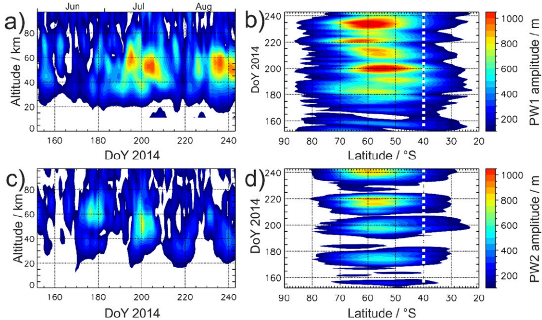
FIG. 11. Geopotential height amplitudes of stationary (a),(b) PW1 and (c),(d) PW2 as (left) a function of height and time averaged between 35° and 45°S and (right) a function of latitude and time averaged between 30- and 40-km altitude.
