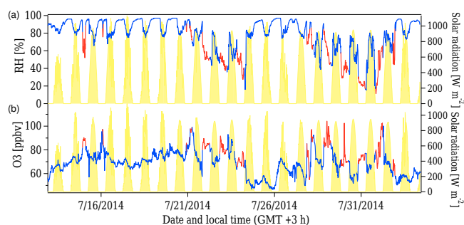
Figure 7. Ozone in ppbv, relative humidity in % and solar radiation in W m -2 (10 min mean values). The red data points are influenced by air masses from the residual layer/free troposphere.
