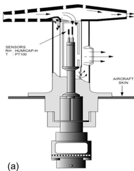
Figure 1: a) Schematic scheme of the temperature sensor attached to the humidity sensor mounted in the Rosemount housing (Helten, 1998). b) Packages 1 and 2 installed aboard the AIRBUS A340-300, and the inlet plate including the Rosemount housing (photograph by courtesy of Lufthansa).
