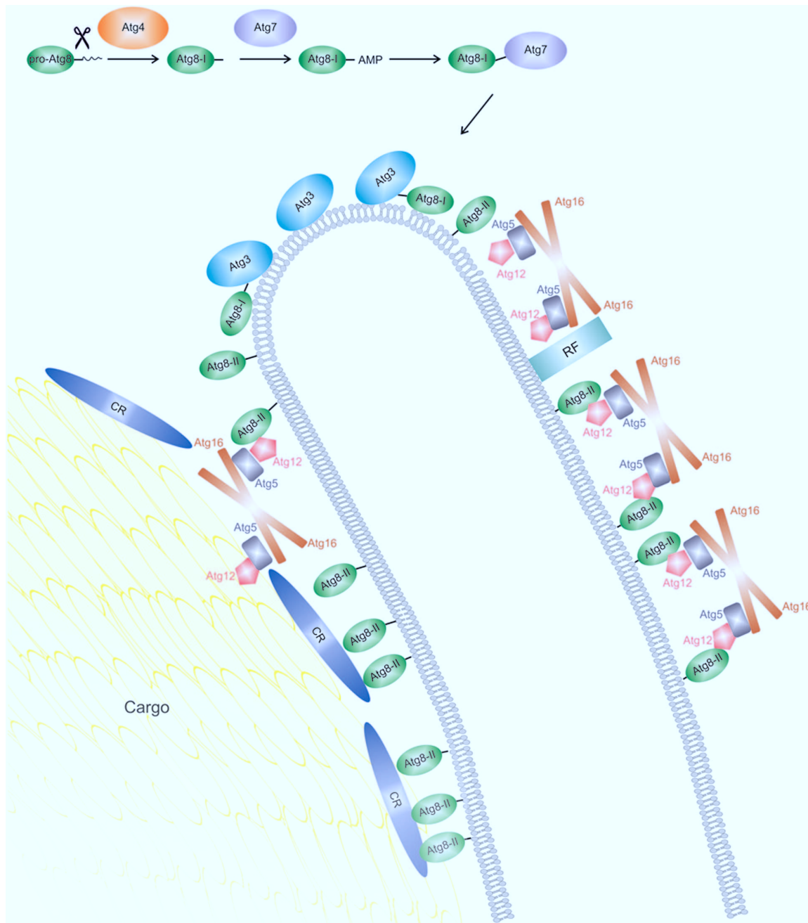
FIGURE 2 | An Atg8-centric view on phagophore expansion around cargo in selective autophagy. Newly expressed Atg8 molecules (pro-Atg8) are cleaved C-terminally by Atg4, yielding a so-called form I (Atg8-I). The latter is activated by the E1-like enzyme Atg7 and transferred to the E2-like Atg3. Formation of the PE conjugate (form II, also termed Atg8-II or Atg8-PE) in vivo requires the Atg12–Atg5–Atg16 complex and is hypothesized to mainly occur in the rim region due to the curvature sensitivity of Atg3. Atg12–Atg5–Atg16 is recruited to the phagophore membrane by specific interaction partners; on the outer surface, these are typically PI3P binding proteins (labeled here recruiting factors, RF), while on the inner surface, cargo receptors (CRs) appear to take over this function. Lipidated Atg8 enables Atg12–Atg5–Atg16 to establish a mesh-like coat on the outer surface, which has been proposed to stabilize the shape of the organelle. On the inside, Atg8 proteins are chiefly responsible for high-avidity binding of degradation targets via cargo receptors, resulting in close apposition of the membrane.
