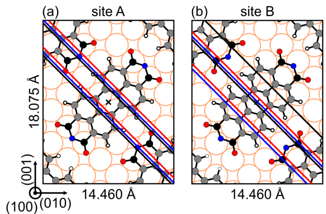
FIG. 11. Superstructure unit cell of PTCDA on Cu(100), plotted for adsorption sites A (a) and B (b). The colored lines, which are lattice periodic and identical in (a) and (b), indicate all positions of the molecular center (black cross) that are compatible with the coherent positions [(111) reflection] of the species of the corresponding color: anhydride oxygen—blue, carboxylic oxygen—red, and functional carbon (C1)—black. Evidently, adsorption site B is in agreement with experimental results.
