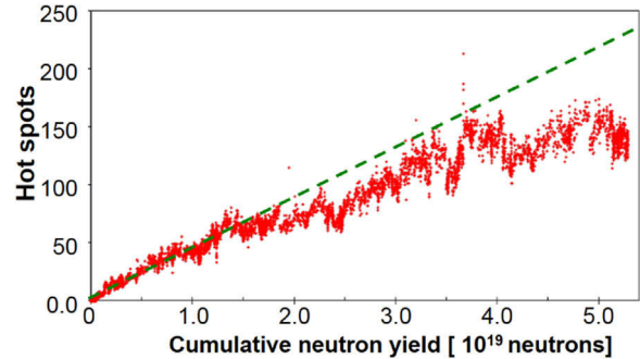
Fig. 5. Hot spots as function of cumulative neutron yield on the uncooled camera used for operation.
