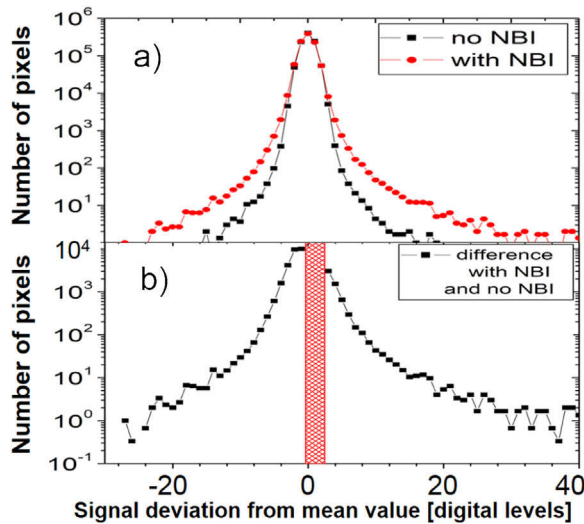
Fig. 6. a) Daynami evolution of hot pixels during the NBI phase and during the ohmic phase of the typical JET 15 MW NBI plasma pulse. b) gives the difference between two distributions shown in Fig. 6a.
