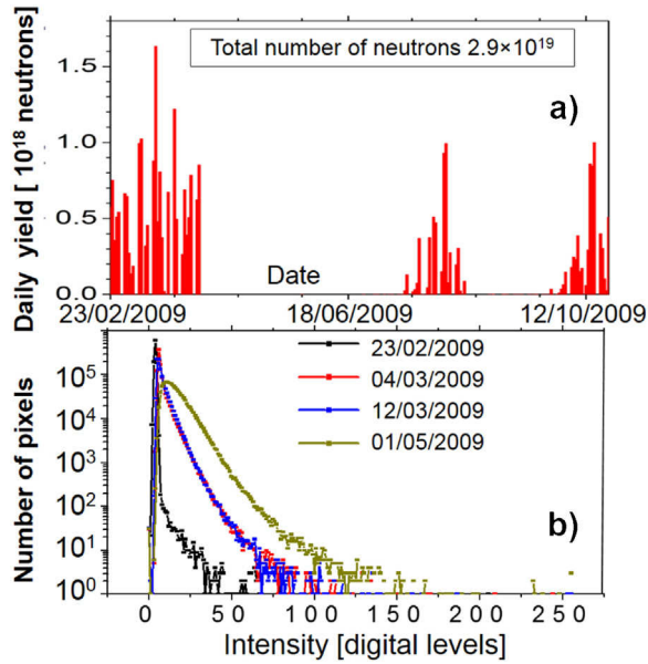
Fig. 3. a) the daily neutron yield during the testing period b) histograms of pixel brightness at four selected times during the test.
