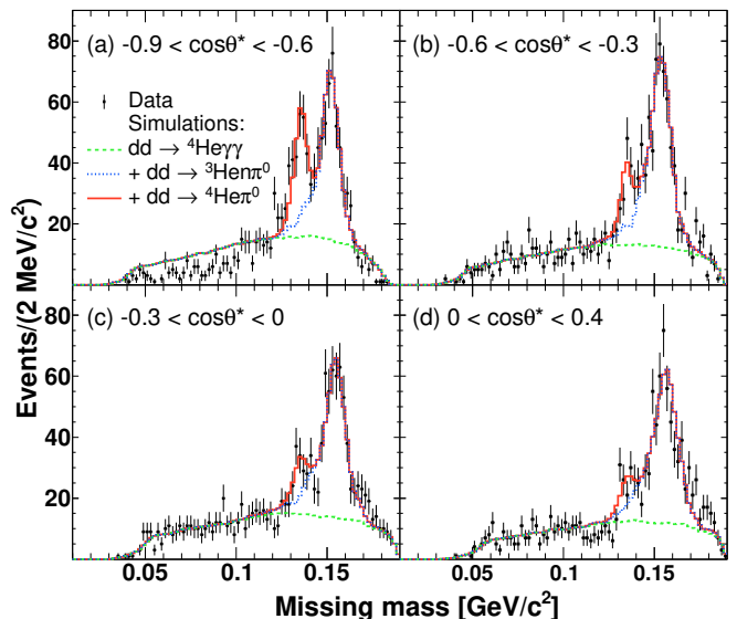
FIG. 1. Missing mass for the dd \rightarrow {}^4\text{He}X reaction for the four angular bins of the production angle of the pion in the center-of-mass system. The spectrum is fitted with a linear combination of the simulated signal and background reactions: double radiative capture dd \rightarrow {}^4\text{He}\gamma\gamma (green dashed line), plus dd \rightarrow {}^3\text{He}\pi^0 (blue dotted line), plus dd \rightarrow {}^4\text{He}\pi^0 (red solid line). The fit excludes the missing mass region below 0.11 \text{ GeV}/c^2 .
