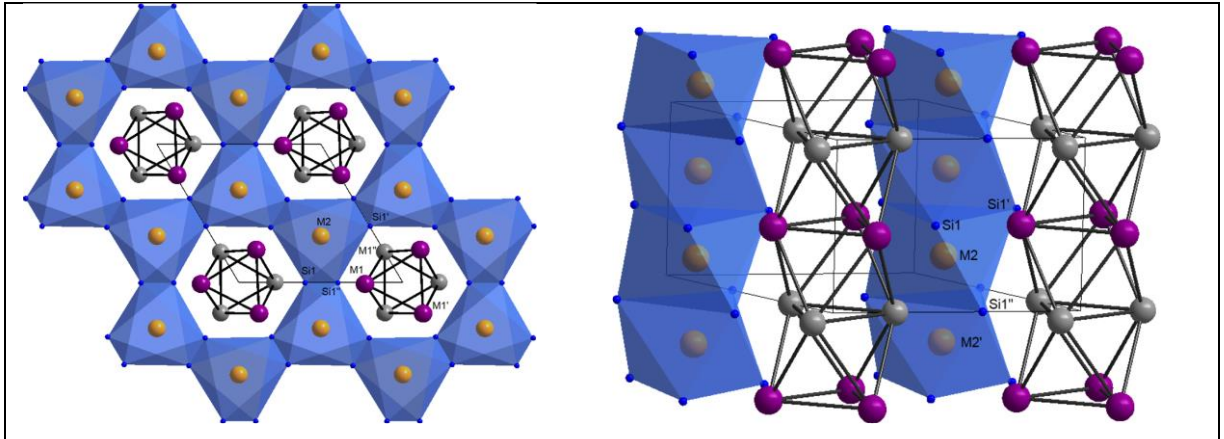
Figure 2.7: Projection of the structure of MnFe_4Si_3 in space group P\bar{6} at 380 K along the [001] -direction (left) and along the [120] -direction (right) [Hering et al., 2015].
