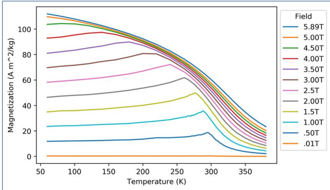
Figure 4.9: Temperature-dependent magnetization of \text{MnFe}_4\text{Si}_3 from hysteresis measurements ( H \parallel [001] )
