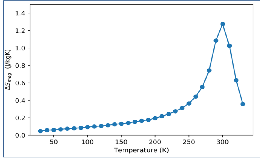
Figure 4.10: MCE of \text{MnFe}_4\text{Si}_3 calculated from the temperature-dependent magnetization at a field of 1T ( H \parallel [100] ).
