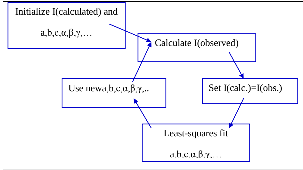
Figure 2.6: Flow chart of the Le Bail process.
