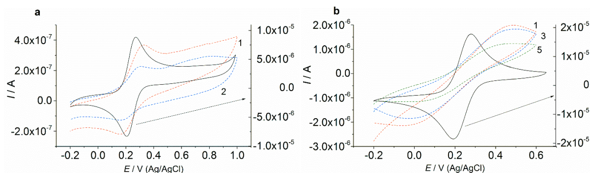
Fig. 5 a, b Cyclic voltammogramms of: a – ferrocenemethanol, 5 \cdot 10^{-5} M, scans 1 and 2; b – hexacyanoferrate(III), 1 \cdot 10^{-3} M, scans 1,3,5, Au NWs on Si/SiO 2 . Black solid lines with a right-hand Y-scale in a , b are CVs on a Si/SiO 2 /Au thin-film gold electrode of 5 \cdot 10^{-4} M ferrocenemethanol and 1 \cdot 10^{-3} M hexacyanoferrate(III), respectively. Background electrolyte: 0.1 M KNO 3 , scan rate rate 0.02 \text{ V s}^{-1}
