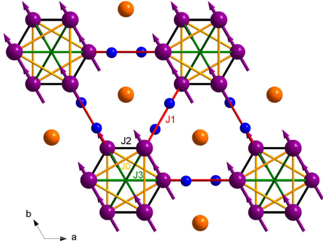
FIG. 1. Projection on the hexagonal plane of the crystal structure of \text{MnFe}_4\text{Si}_3 in P6_3/mcm space group. Sites occupied by Mn and Fe (WP 6g, large magenta) carry magnetic moments 1.5 \mu_B parallel to b axis; sites occupied by Fe (WP 4d, large yellow) and Si atoms (small blue) carry no magnetic moments. Yellow lines ( J_0 ) connect atoms in the same plane, red lines ( J_1 ), black lines ( J_2 ), and green lines ( J_3 ) in different planes.
