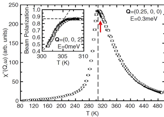
FIG. 5. Temperature dependence of dynamical spin susceptibility \chi''(\mathbf{Q}, \omega) at \mathbf{Q} = (0.25, 0, 0) and E = 0.3 meV measured with unpolarized neutrons at IN12. The dashed vertical line and the red arrow indicate T_C \approx 305 K and 1.036T_C \approx 316 K, respectively. The inset shows the temperature dependence of the beam polarization at \mathbf{Q} = (0, 0, 2) Bragg peak.
