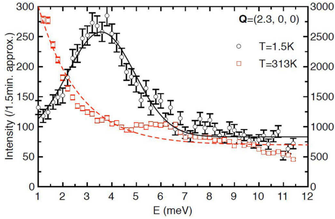
FIG. 2. Energy spectra at \mathbf{Q} = (2.3, 0, 0) measured at IN12 spectrometer with unpolarized setup at 313 K (squares) and 1.5 K (circles). Neutron intensity for data at 1.5 K and 313 K is given on the left and right vertical axis, respectively. The solid line corresponds to a Gaussian function fit and the dashed line is a guide for the eyes.
