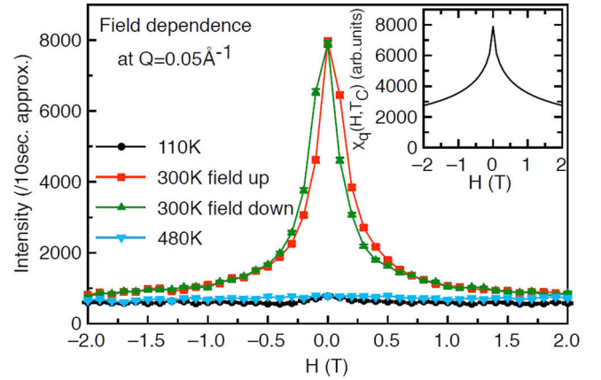
FIG. 6. Evolution of elastic scattering at Q = 0.05 \text{ \AA}^{-1} measured at MIRA as a function of magnetic field at three temperatures. Lines can be used as guides for the eyes. The inset shows a calculation of the field dependence of \chi_q(H, T_C) following Ref. [19].
