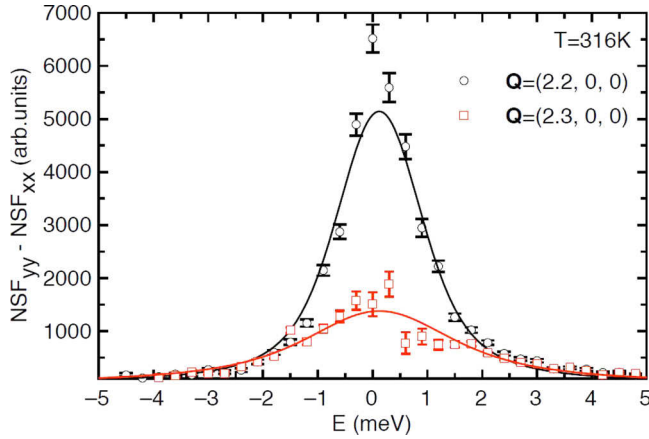
FIG. 7. Spin fluctuations \langle \delta M_c \rangle obtained at IN22 and measured at \mathbf{Q} = (2.2, 0, 0) (black circles) and \mathbf{Q} = (2.3, 0, 0) (red squares) at 1.036T_C . Solid lines represent fits as explained in the text.
