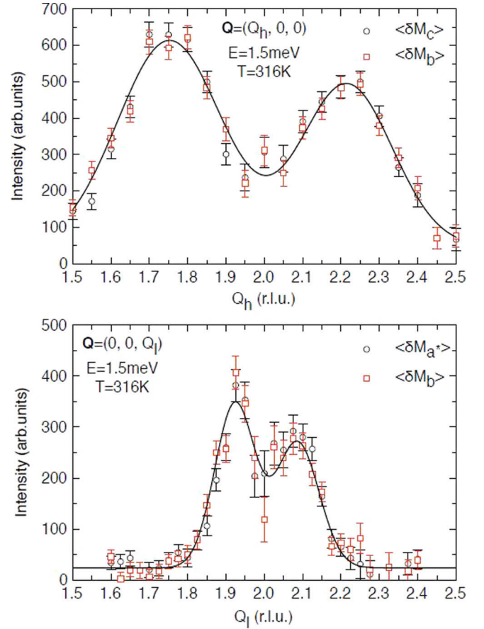
FIG. 9. Subtracted spin fluctuations spectra from constant energy scans at 1.5 meV at 316 K along (h00) (top) and (00l) (bottom) directions obtained at IN22. The indices i in \langle \delta M_i \rangle indicates the direction of fluctuations ( a^* , b , and c ). Solid lines correspond to fits with Lorentzian functions.
