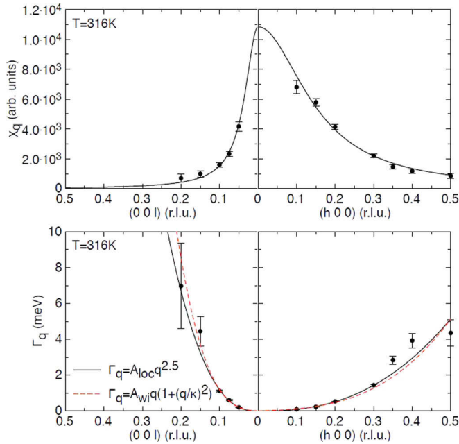
FIG. 8. q -dependent susceptibility \chi_q (top) and linewidth \Gamma_q (bottom) in the (00l) and (h00) directions at 316 K. The solid black lines for \chi_q correspond to Lorentzian fits as described in the text. The solid black and dashed red line for \Gamma_q correspond to the localized and weak itinerant model of ferromagnetism, respectively.
