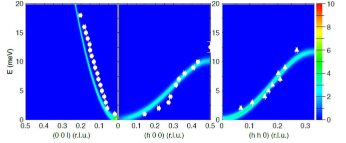
FIG. 4. Magnon dispersion at T = 1.5 K along (00l), (h00), and (hh0) directions from polarized (circles) and unpolarized (triangles) INS measurements. The color-coded intensity corresponds to spin-wave simulation as described in the text.
