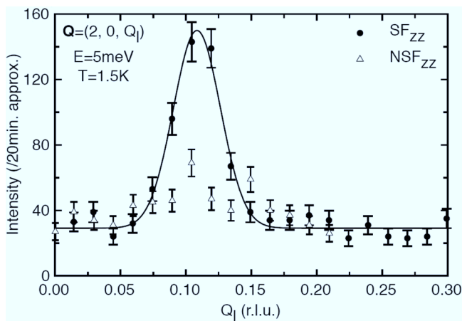
FIG. 3. Polarized inelastic neutron scattering spectra obtained at IN12 around \mathbf{Q} = (2, 0, Q_l) at constant energy transfer of 5 meV at T = 1.5 K from spin flip and non-spin flip channel. The solid line represents a fit with a Gaussian function.
