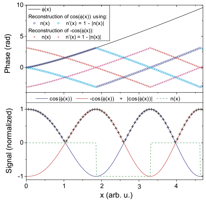
Fig. 8. Illustration of recovery of the one-dimensional phase \phi(x) from the DEEH amplitude |\cos(\phi(x))| . The top panel shows the original phase (black solid line) and variants of its recovery (circles and crosses). The bottom panel shows the amplitude signal (black crosses) and variants of its inversion (blue and red solid lines). Depending on the definition of n(x) (green dashed line in lower graph) and on the inversion of the cosine function (red and blue solid lines), the result of phase recovery can either match the input signal (blue circles in the upper graph) or not provide a match (cyan circles and crosses). (For interpretation of the references to color in this figure legend, the reader is referred to the web version of this article.)
