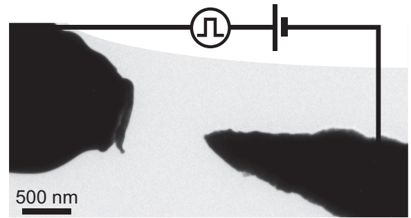
Fig. 1. Bright-field TEM micrograph of the ends of two metallic needles mounted in a Nanofactory specimen holder, overlaid with a schematic circuit diagram showing how a voltage is applied between them in situ in the TEM.
