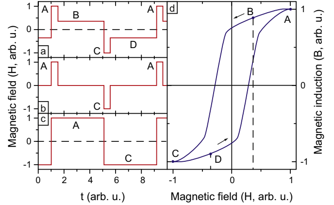
Fig. 12. Schematic representation of a quasi-static magnetic switching experiment. Panels (a–c) show possible sequences of applied pulses as a function of time t . Panel (d) shows the hysteresis curve of the specimen. The applied pulses can be used to access: (a) arbitrary points B and D in the hysteresis cycle; (b) remanent states and (c) saturated states.
