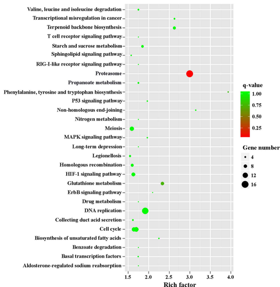
Fig. 10 The top 30 of KEGG enrichment of significant upregulated genes in MZ-2
