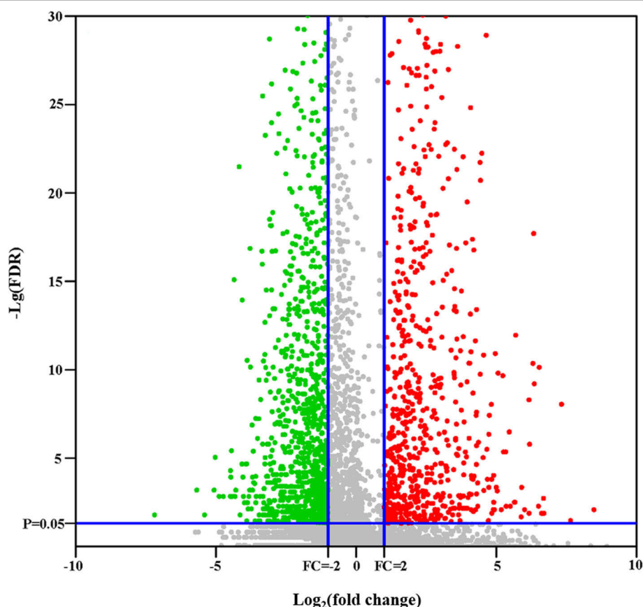
Fig. 1 Volcano plots of up/downregulated and not differentially expressed unigenes between MZ-2 and MZ-3. Unigenes differentially expressed level: the unigenes are significantly upregulated (red spot), downregulated (green spot), and no difference (grey spot)
