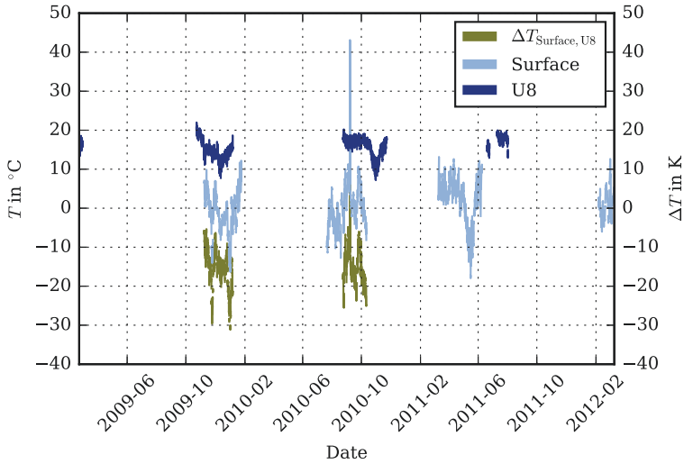
Figure 3.2: Winter conditions: time series of underground (U8) and surface temperatures and corresponding differences for coincident data.
