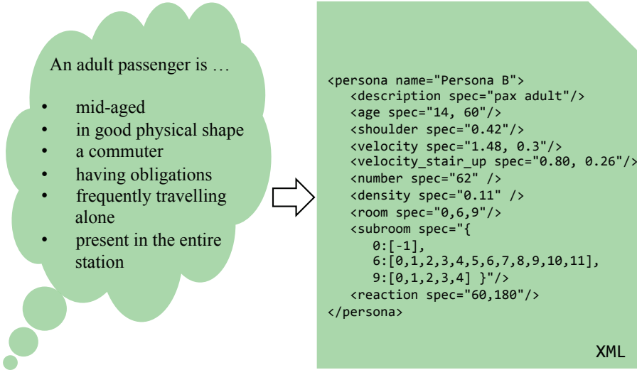
Figure 5.4: Exemplary translation of narrative persona characteristics into numeric values.
