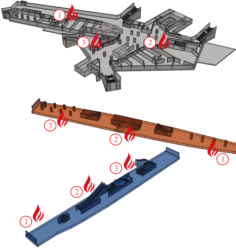
Figure 4.3: Distribution of nine fire locations across the station.
