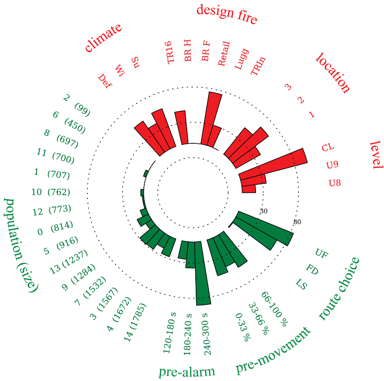
Figure C.10: Radar plot illustrating the parametric origin of cluster G.
