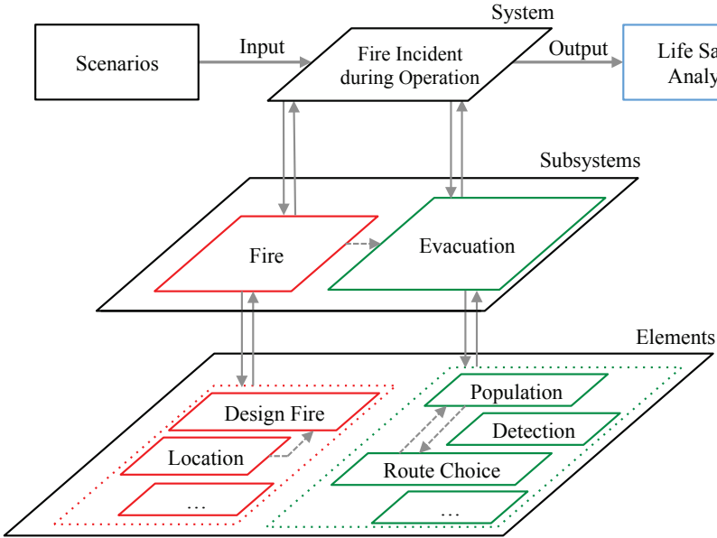
Figure 2.1: Schematic system definition for life safety analysis in case of fire. Based on [Winzer, 2013, p. 69].
