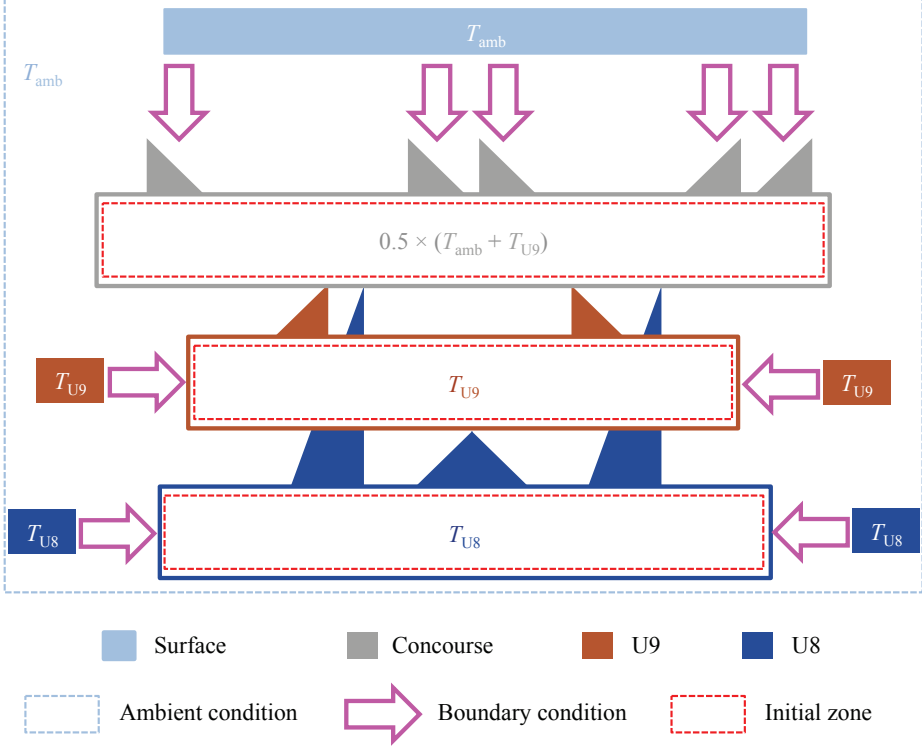
Figure 3.1: Overview of the climate model utilising ambient, initial, and boundary temperature conditions throughout the station. The triangles illustrate the staircases.
