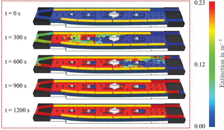
Figure 4.9: Two-dimensional slices through the U8 level aligned with the floor and visualising the state of extinction over a period of 20 minutes. Red areas indicate extinction coefficients greater than 0.23 \text{ m}^{-1} .
