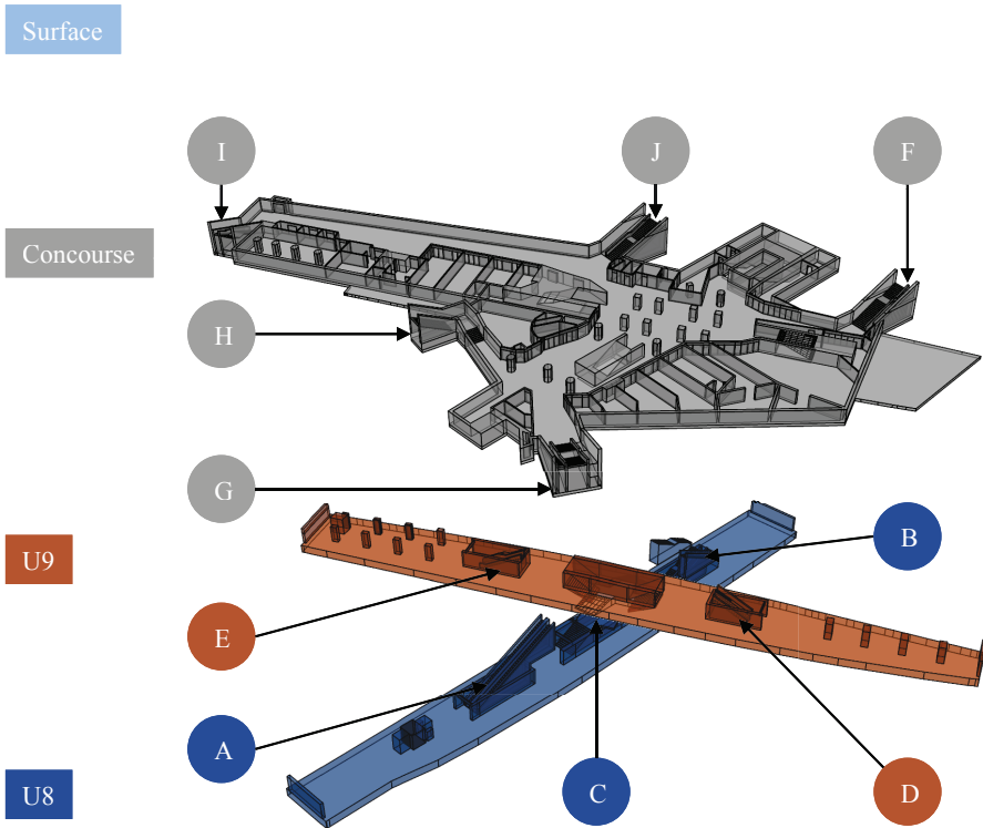
Figure 1.1: Schematic overview of the station.
