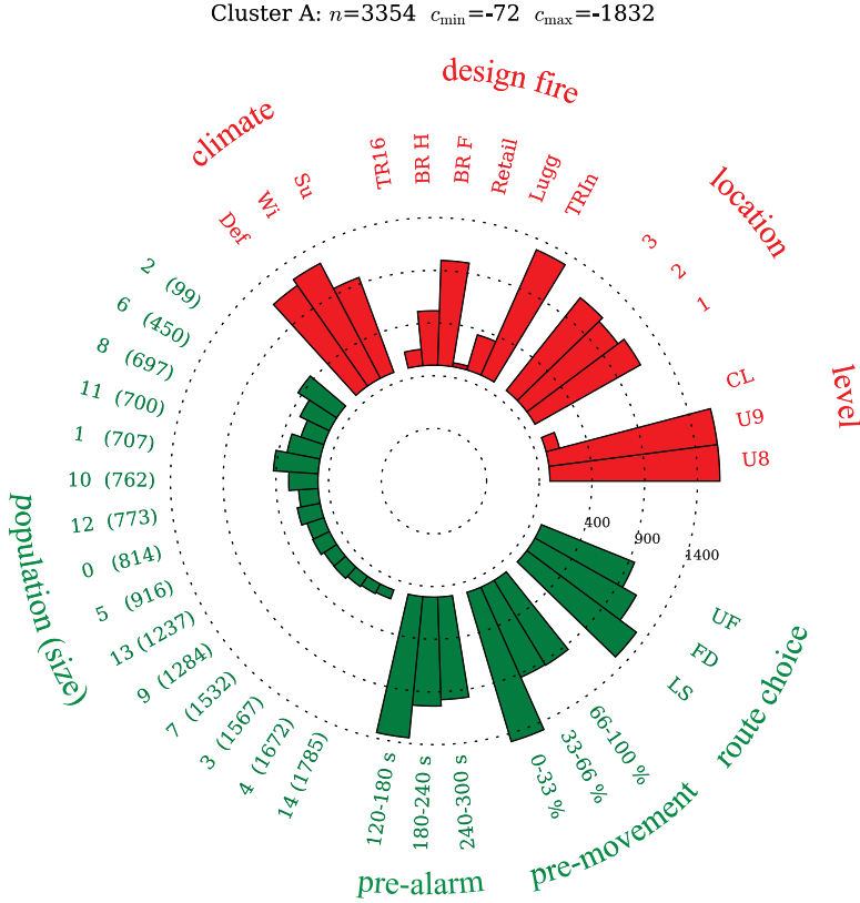
Figure 6.10: Radar plot illustrating the parametric origin of cluster A.
