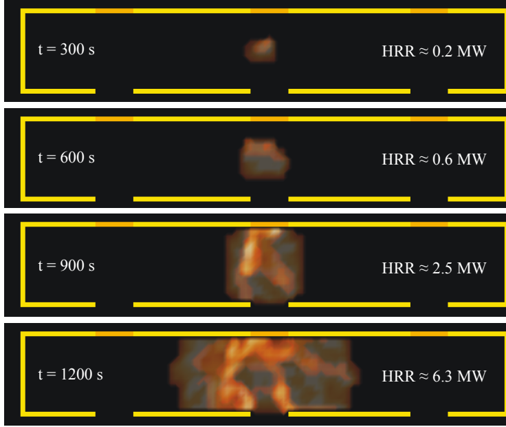
Figure 4.2: Top view of time, flame spread, and corresponding heat release rate in a carriage applicable to the design fire BR F .
