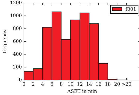
Figure 4.12: Histogram showing the frequencies of ASET in the U8 level applicable for the fire scenario f001.
