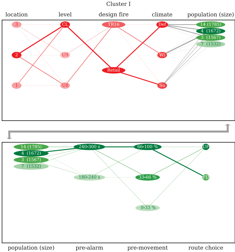
Figure C.17: Parallel coordinate plot illustrating the parametric relations of cluster I.
