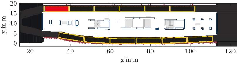
Figure 4.8: Top view on the U8 level. Four staircases connect the platform with the U9 level. Both tracks are occupied by a six-car trainset. The seat of fire is assumed in the carriage marked red.
