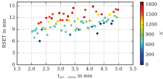
Figure 5.15: Reference occupant scenario ensemble: impact of pre-alarm time on RSET .
