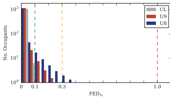
Figure C.3: FED histogram of scenario cluster C.
