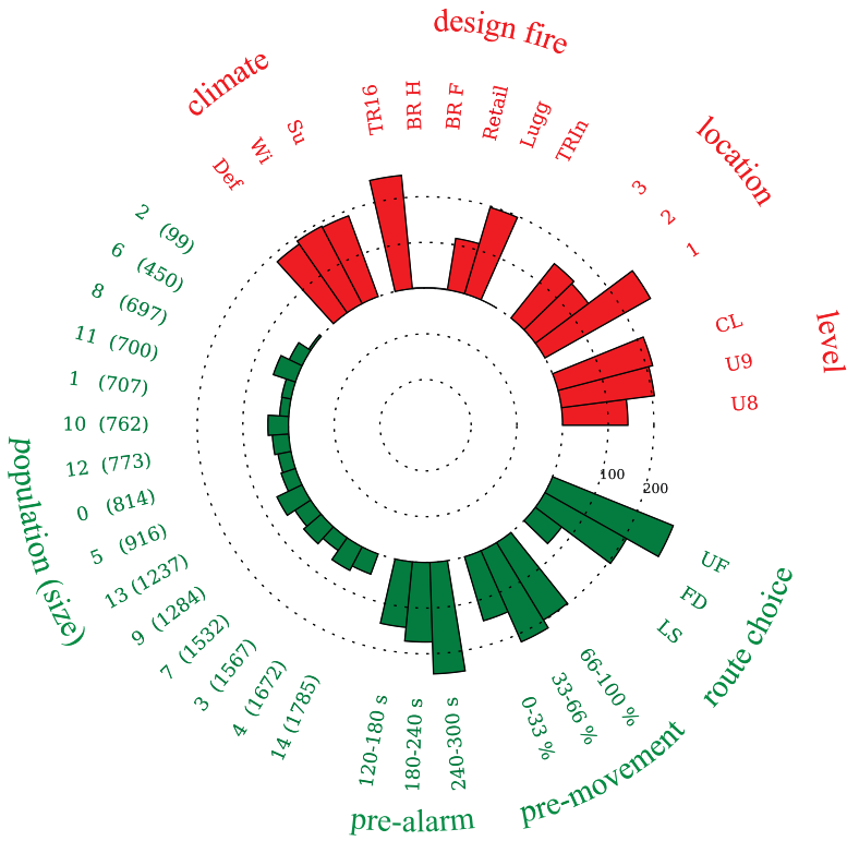
Figure C.4: Radar plot illustrating the parametric origin of cluster D.
