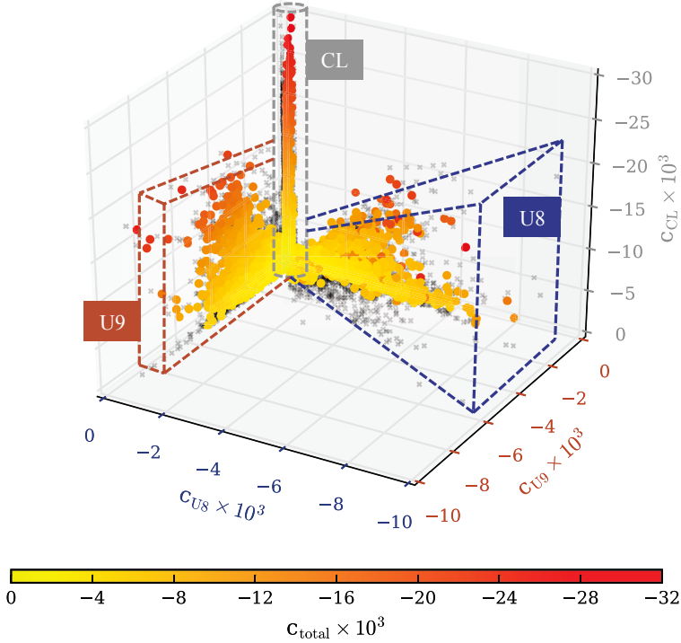
Figure 6.7: Single consequences observed on the levels U8, U9, CL, and the resulting total consequences. Scatter points represent scenario combinations and grey crosses illustrate their projection to the plains for better spatial comprehension. The dashed enclosures demonstrate the influence of the level where a fire is assumed. Note: z -axis is not to scale.
