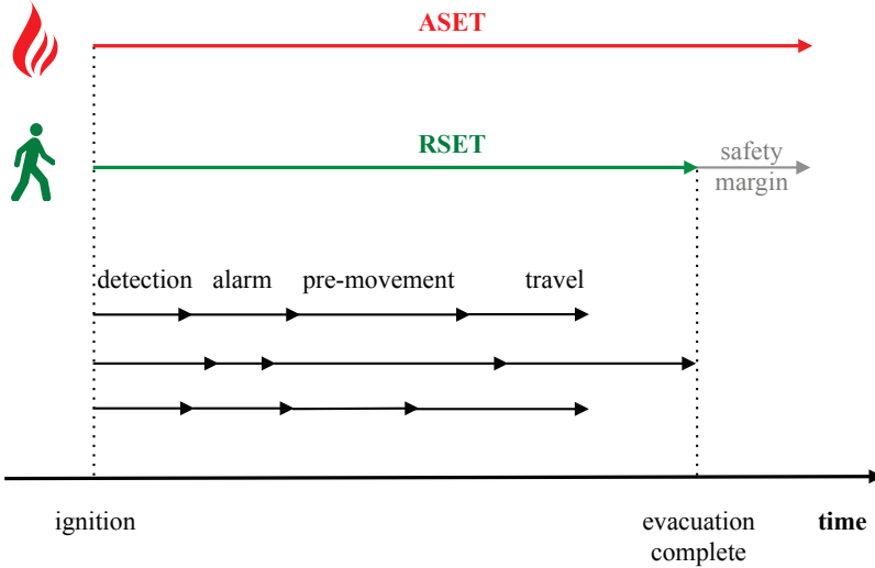
Figure 2.3: Summary of the ASET-RSET concept. In orientation to [Gwynnee and Boyce, 2016].
