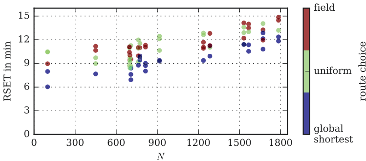
Figure 5.16: Reference occupant scenario ensemble: impact of route choice on RSET .
