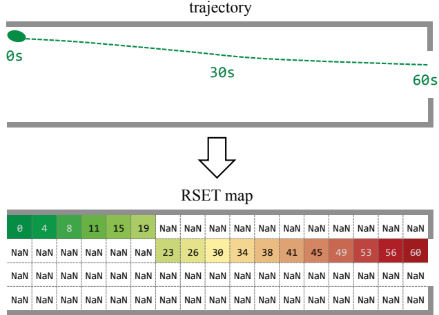
Figure 5.11: RSET map generation on the basis of a pedestrian's trajectory.
