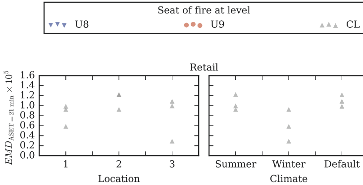
Figure 4.16: Separated analysis of medium-energetic design fires regarding the impact of fire locations and climatic conditions on the EMD .
