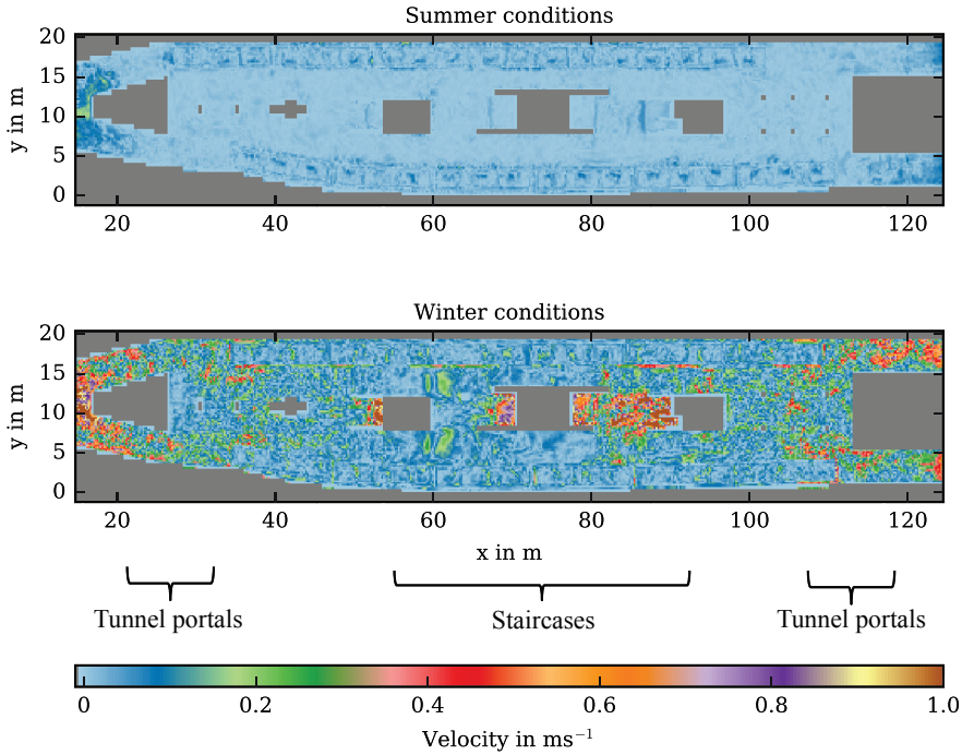
Figure 3.5: Horizontal slices of absolute velocities for summer and winter conditions. The slices refer to the U8 level at a height of 1.95 m after 600 s. For the winter case, velocities greater than 1 \text{ m s}^{-1} have established in proximity to the tunnel portals and upward staircases.
