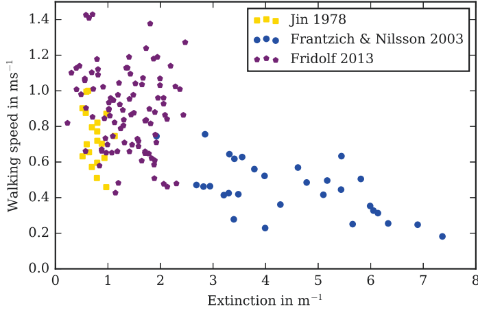
Figure 3.10: Experimental studies on the relation of extinction coefficient and walking speed applicable to non-irritant smoke.
