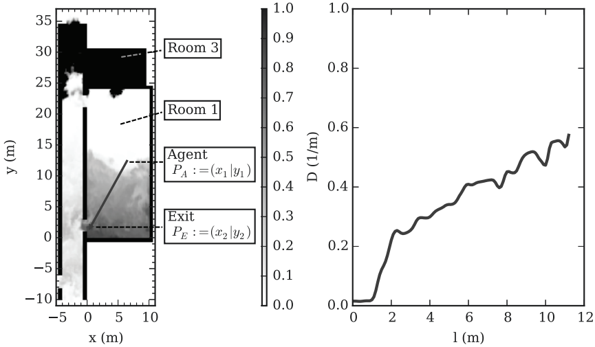
Figure 3.8: Extraction of optical density from fire simulation data with the help of spline interpolation.
