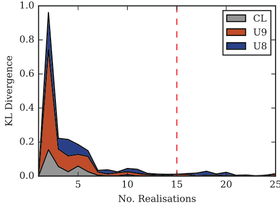
Figure 5.1: Development of Kullback-Leibler Divergence for RSET probability density functions with increasing numbers of realisations.
