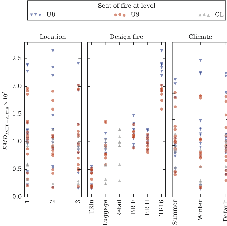
Figure 4.14: Scatter matrix illustrating the impact of the fire scenario parameters location, design fire, and climate on the EMD . Design fires are ordered by total heat release.
