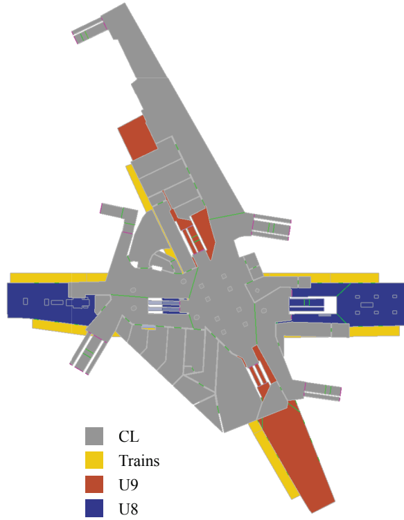
Figure 5.2: Vertex-based geometry of Osloer Straße including the levels U8, U9, CL, and three trains. Magenta lines illustrate transitions between rooms and green lines represent crossings between subrooms.
