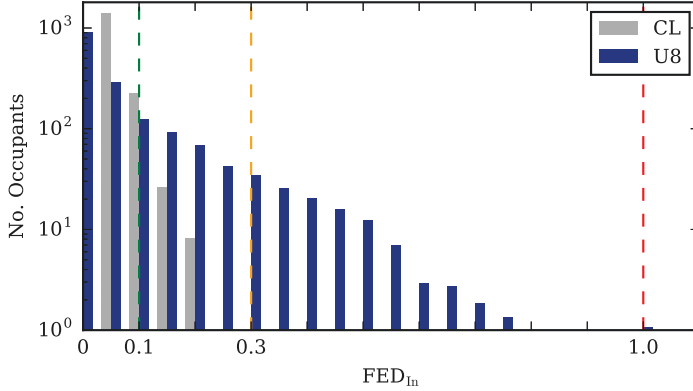
Figure 6.21: FED histogram of scenario cluster J.
