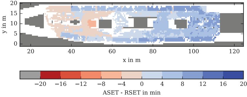
Figure 6.3: Exemplary difference map unifying ASET and RSET . The colour map has been discretised into intervals of four minutes. Grey fields represent areas that are obstructed by the built environment. White areas have not been traversed at all.
