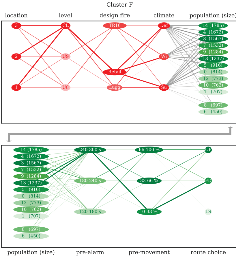
Figure 6.15: Parallel coordinate plot illustrating the parametric relations of cluster F.
