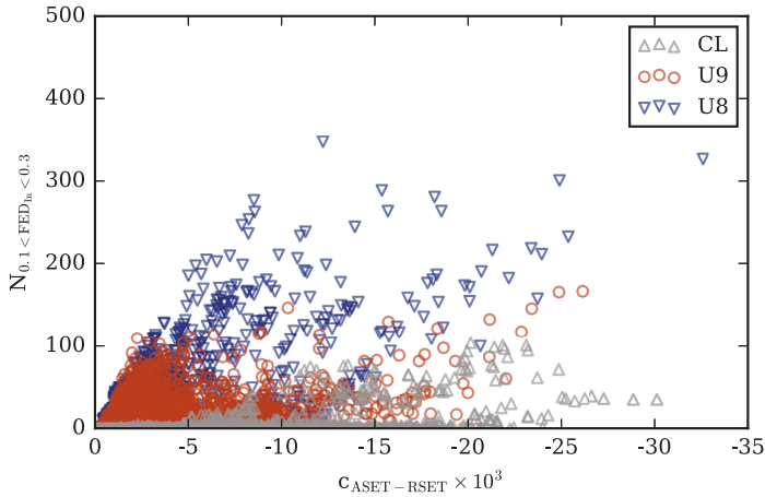
Figure 6.22: Correspondence of ASET-RSET analysis and FED analysis applicable to 0.1 < FED_{In} < 0.3 .
