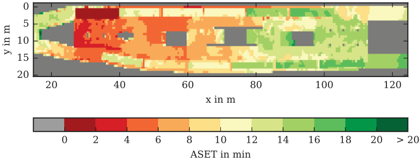
Figure 4.11: Consolidated ASET map derived from the entire set of incorporated quantities. Applicable for the U8 level and the fire scenario f001.
