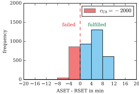
Figure 6.5: Quantification of consequences based on ASET-RSET difference map distribution applicable to the U8 level.
