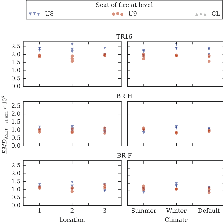
Figure 4.15: Separated analysis of high-energetic design fires regarding the impact of fire locations and climatic conditions on the EMD .
