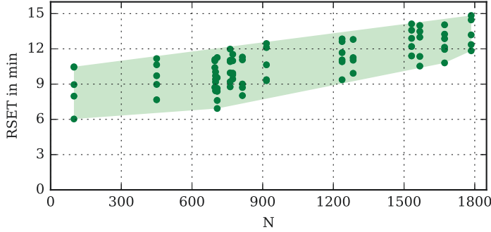
Figure 5.14: Reference occupant scenario ensemble: correlation of occupant number and RSET . The light green polygon illustrates the margin in which RSET is expected to range.
