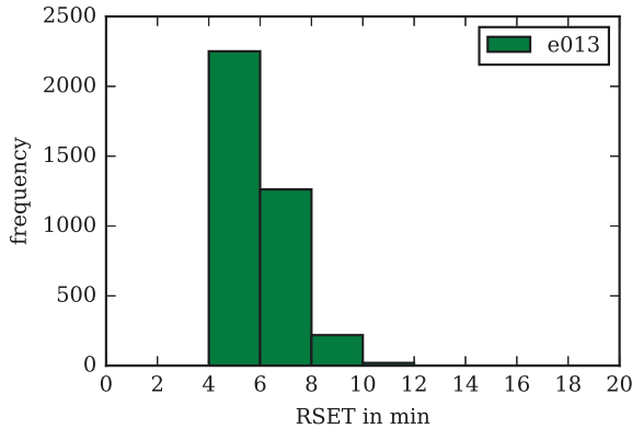
Figure 5.13: Distribution of the ninety-fifth percentile of RSET in the U8 level.
