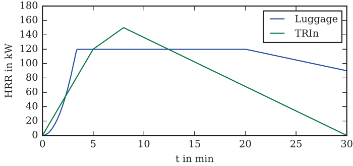
Figure 4.6: Low-energetic design fires representing a burning luggage item ( Luggage ) and a self-extinguishing fire inside a rail car ( TRIn ).
