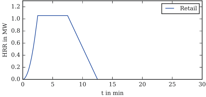
Figure 4.5: Medium-energetic design fire represented by a sprinklered retail unit fire ( Retail ).
