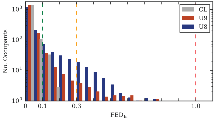
Figure C.15: FED histogram of scenario cluster H.
