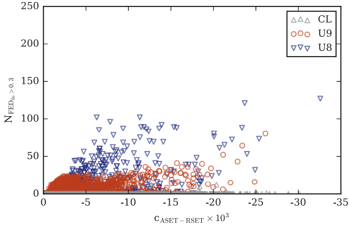
Figure 6.23: Correspondence of ASET-RSET analysis and FED analysis applicable to FED_{In} > 0.3 .
