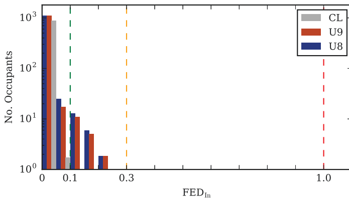
Figure 6.19: FED histogram of scenario cluster B.
