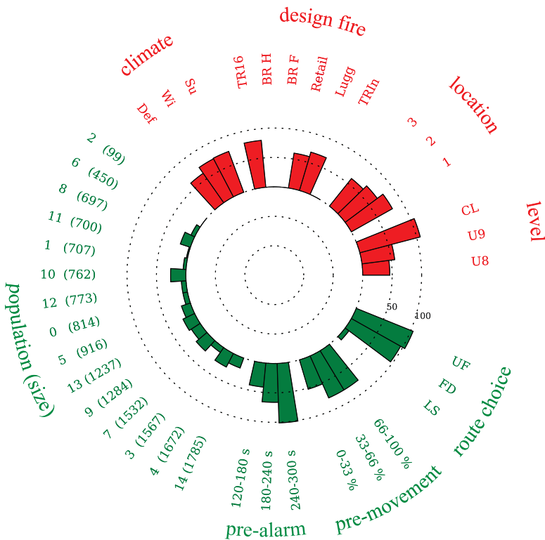
Figure C.7: Radar plot illustrating the parametric origin of cluster E.
