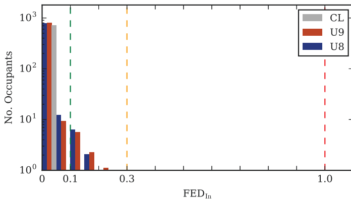
Figure 6.18: FED histogram of scenario cluster A.
