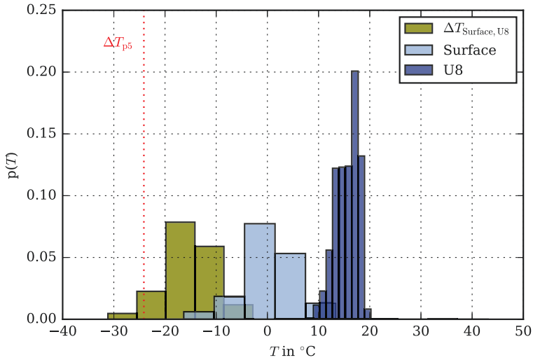
Figure 3.3: Winter conditions: distributions of underground (U8) and surface temperatures and corresponding difference when data series have been coincident. The dashed line illustrates the fifth percentile boundary, which has been applied to extract the most distinct temperature differences between surface and underground.
