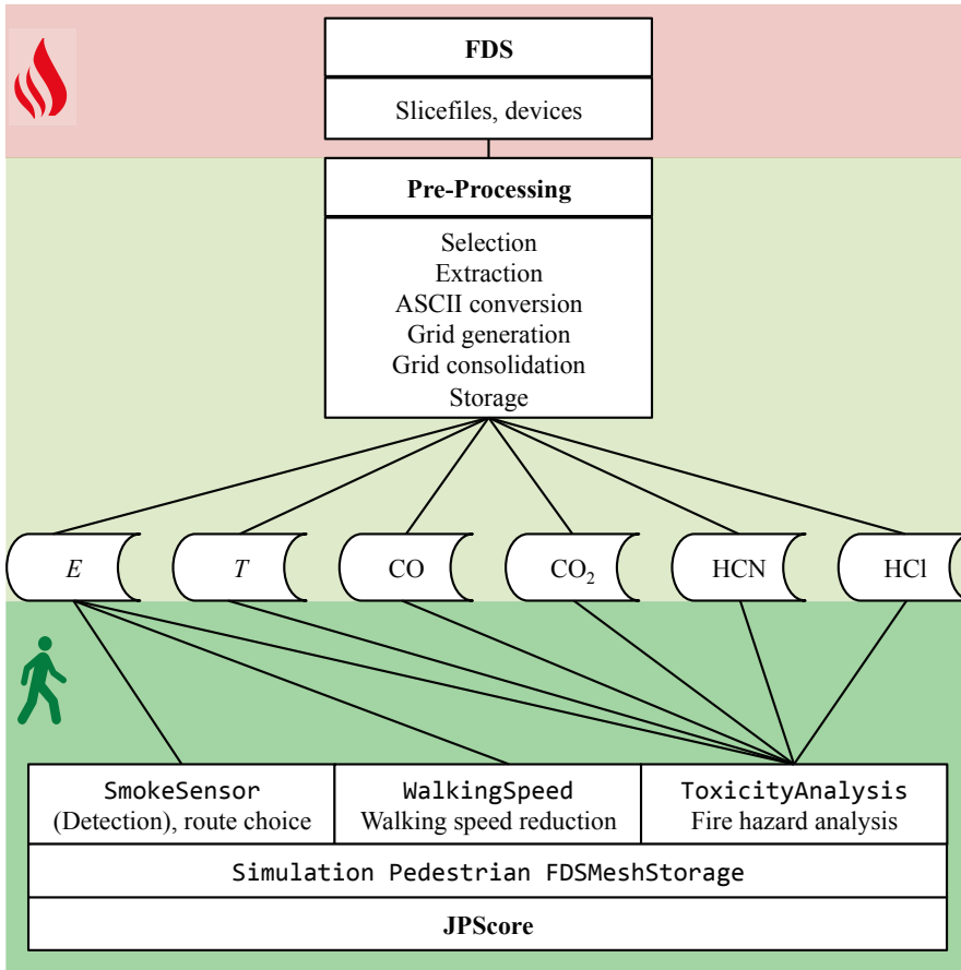
Figure 3.7: Overview of hierarchy and main functionalities of JPSfire , processed fire simulation data, and supplied classes of JPScore .
