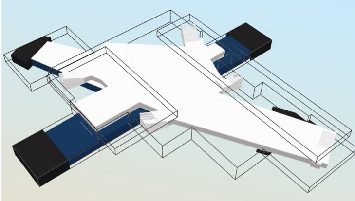
Figure 4.1: Decomposition of the computational domain into 12 meshes.
