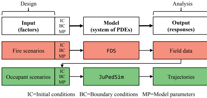
Figure 2.7: General overview of design and analysis of simulation experiments and its application within this study.
