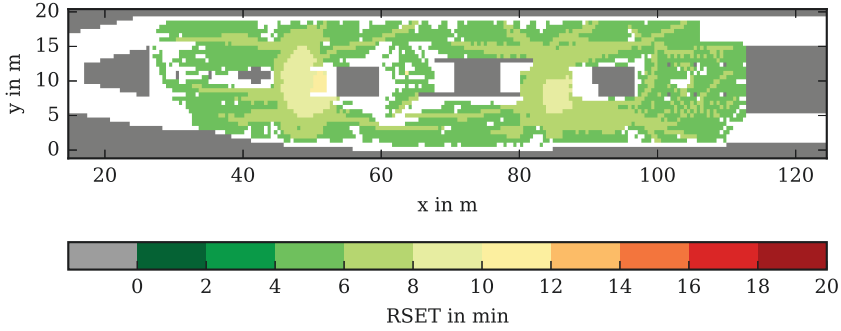
Figure 5.12: Exemplary map illustrating the ninety-fifth percentile of RSET in the U8 level. The colour map has been discretised into intervals of two minutes. Grey fields represent areas that are obstructed by the built environment. White areas have not been traversed at all.
