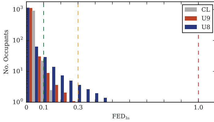
Figure C.6: FED histogram of scenario cluster D.
