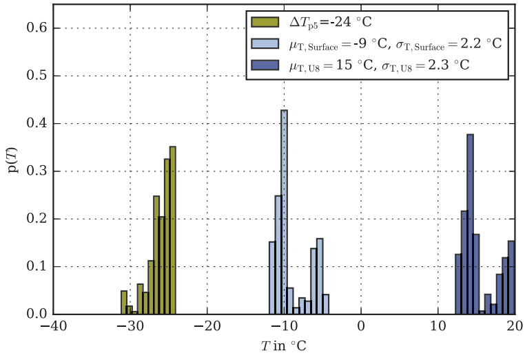
Figure 3.4: Winter conditions: illustration of temperature difference distribution bounded by the fifth percentile and the underlying components of underground (U8) and surface temperature.
