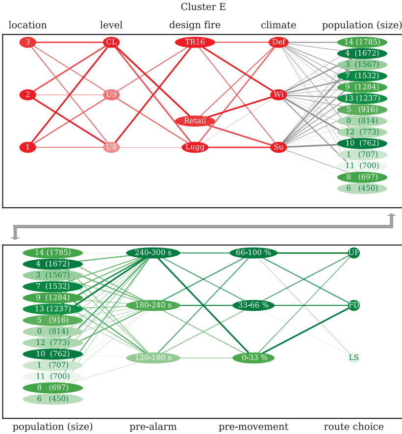
Figure C.8: Parallel coordinate plot illustrating the parametric relations of cluster E.
