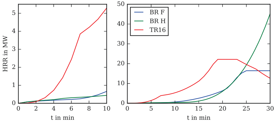
Figure 4.4: High-energetic design fires including BVG vehicle generations BR F , BR H , and the generalised TR16 envelope curve.
