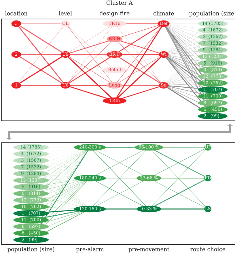
Figure 6.11: Parallel coordinate plot illustrating the parametric relations of cluster A.
