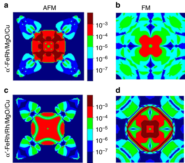
Fig. 4 Transmission distribution in two-dimensional Brillouin zone for \alpha' -FeRh/MgO(2.5 u.c.)/Cu and \alpha' -FeRh/Rh(1 u.c.)/MgO(2.5 u.c.)/Cu junctions at Fermi level. a, b Minority-spin channels at AFM and FM states for \alpha' -FeRh/MgO/Cu junctions. c, d Minority-spin channels at AFM and FM states for \alpha' -FeRh/Rh/MgO/Cu junctions
