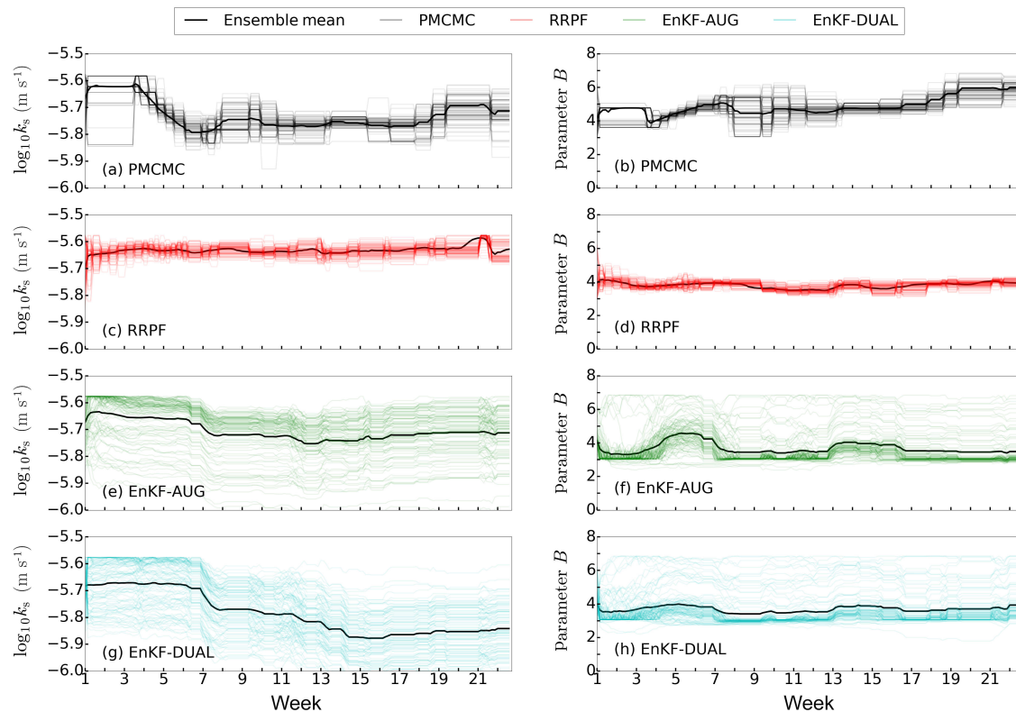
Figure 11. Sampled trajectories of the N = 100 ensemble members of the saturated hydraulic conductivity ( \log_{10}k_s in \text{m s}^{-1} ) at 50 cm depth (a, c, e, g) and soil hydraulic parameter B at 50 cm depth (b, d, f, h) of CLM during the 5-month assimilation period of weeks 1 to 22 using (a–b) PMCMC (grey) (c–d) RRPf (red), (e–f) EnKF-AUG (green), and (g–h) EnKF-DUAL (cyan). The solid black line signifies the evolution of the ensemble mean values of \log_{10}k_s and B . Please note that \log_{10}k_s (in \log_{10}(\text{m s}^{-1}) ) and parameter B are derived from the sand, clay, and organic matter fractions of each soil layer, which are estimated during the assimilation period.
