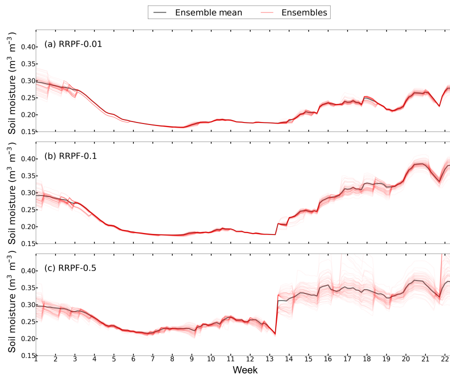
Figure 9. Soil moisture trajectories of the N = 100 ensemble members at 50 cm depth for the 5-month assimilation period (weeks 1 to 22) of the Rollesbroich site using VIC-3L and (a) RRPF-0.01, (b) RRPF-0.1, and (c) RRPF-0.5. The solid black line signifies the ensemble mean soil moisture prediction.
