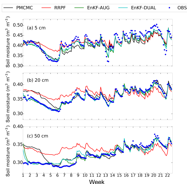
Figure 10. CLM predicted time series of soil moisture content at (a) 5 cm, (b) 20 cm, and (c) 50 cm depth during the 5-month calibration period using PMCMC (black), RRPf (red), EnKF-AUG (green), and EnKF-DUAL (cyan). The first day of week 1 is 1 March 2012 and week 22 starts with 26 July 2012.
