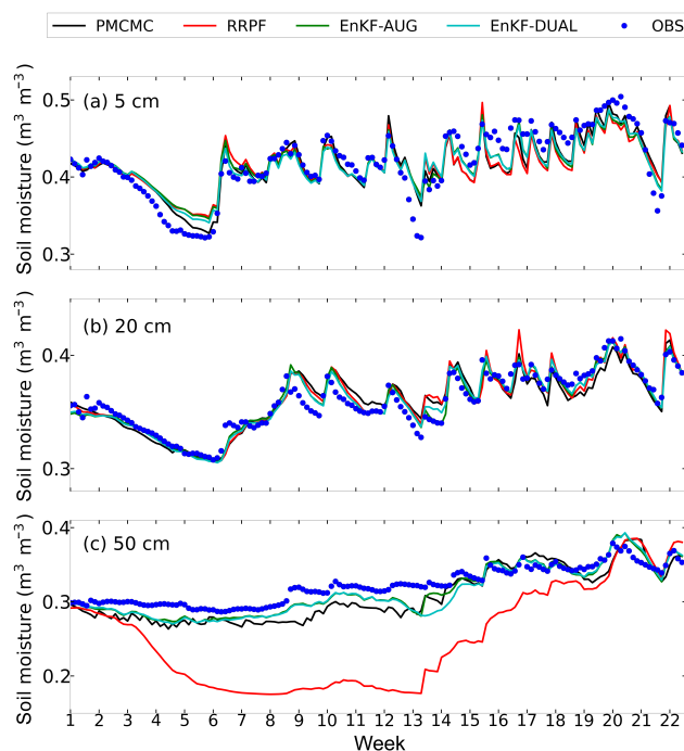
Figure 3. Assimilation period: observed (blue dots) and VIC-3L predicted time series (solid lines) of soil moisture content at depths of (a) 5, (b) 20, and (c) 50 cm in the Rollesbroich site. Color coding is used to differentiate between the results of PMCMC (black), RRPF (red), EnKF-AUG (green), and EnKF-DUAL (cyan). The first days of weeks 1 and 22 are 1 March 2012 and 26 July 2012, respectively.
