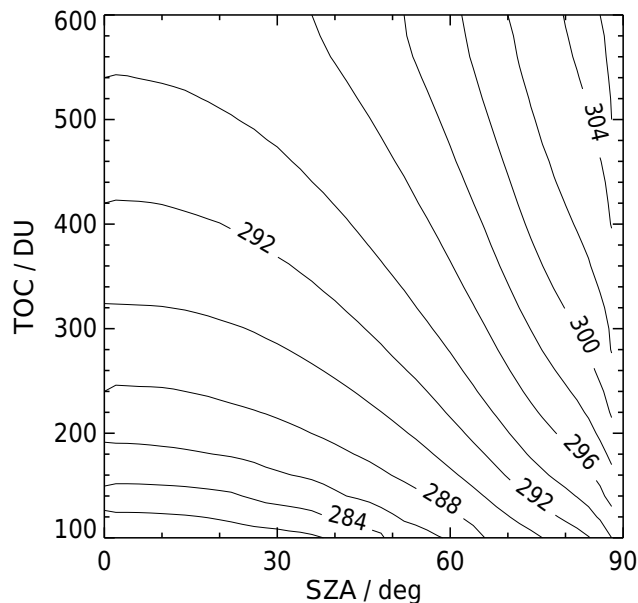
Figure 12. Contour plot of atmospheric cutoff wavelengths (nm) for an altitude of 15 km as a function of the solar zenith angle (SZA) and total ozone column (TOC). The data were derived from radiative transfer calculations of downward clear-sky spectral actinic flux densities defining a lower limit F_{\lambda} \leq 5 \times 10^9 \text{ cm}^{-2} \text{ s}^{-1} \text{ nm}^{-1} . A similar plot for an altitude of 0 km can be found in the Supplement.
