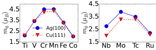
FIG. 1. Calculated ground state spin magnetic moments for several 3d (left) and 4d (right) transition metal adatoms deposited on Ag(100) and Cu(111) denoted by circles (blue) and triangles (red), respectively.
