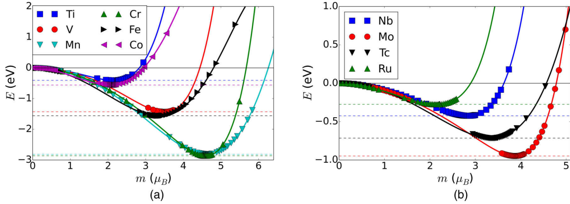
FIG. 4. (a) and (b), calculated energy as a function of the adatom's magnetic moment for 3d and 4d transition metal elements, respectively. DFT calculations are denoted by markers, while the solid lines are a fit to the calculations using E = \sum_{i=2}^8 a_i m^i with only even powers. The horizontal dashed lines mark the minimum energies for different adatoms.
