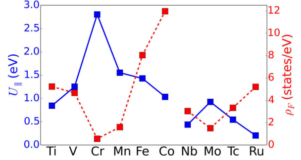
FIG. 3. 3d and 4d magnetic adatoms deposited on Ag(100). Solid (blue) and dashed (red) lines show the calculated values for U_{\parallel} [from Eq. (9)] and \rho_F whose corresponding ordinate axes are placed on the left (blue) and right (red) of the graph, respectively. Note that lines are broken in order to separate 3d from 4d elements.
