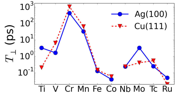
FIG. 8. Calculated values for the transverse relaxation time T_{\perp} for magnetic 3d and 4d adatoms on Ag(100) (blue circles) and Cu(111) (red triangles). Note the logarithmic scale in the y axis.
