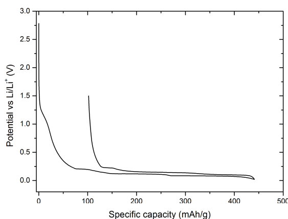
Figure 4. First cycle potential profile of graphite/Li cell containing 1\text{ M LiPF}_6 in EMS:EA (1:1) + 4% FEC electrolyte, in the potential range from 0.02 to 1.5 V vs. \text{Li/Li}^+ .
