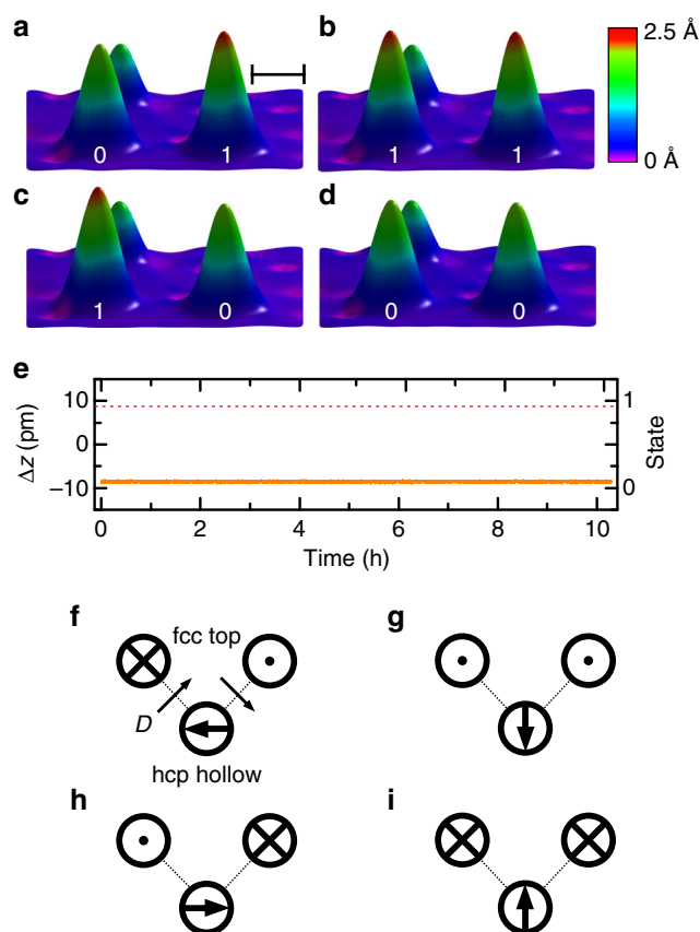
Fig. 5 Two-bit register and four-state memory based on giant moment clusters. a–d Spin-resolved constant-current images of two fcc top clusters in the four possible spin states (01), (11), (10), and (00), where 0 and 1 correspond to downwards and upwards pointing magnetization, respectively (imaging parameters: V = -1 mV, I = 500 pA, B = 0 T, T = 0.3 K). The Fe atom in the back serves as a marker for the apparent height. The scale bar defines a length of 1 nm. Between the images, the tip was positioned on top of the cluster whose state was intended to be changed, the bias was slowly increased until the state switched, and then quickly decreased to the imaging parameter. e The long-term stability of one of the two magnetic bits is shown by measuring the height of the cluster (orange trace) in the state 0 over more than 10 h ( V = -0.7 mV, I = -50 pA, B = 0 T, T = 0.3 K), without a single switch into the state 1, whose height reference is given by the red dotted line, which was determined from the magnetic contrast in images a–d . f–i , Top view schematic diagram of a possible memory with four different realized spin states on a hcp hollow cluster. The two upper circles in each panel illustrate two fcc top clusters prepared in magnetization states up (dot) or down (cross). The lower circle in each panel signifies a hcp hollow cluster (or a hcp atom), which is forced into one of the four spin states indicated by the thick arrow, as dictated by the Dzyaloshinskii-Moriya interaction D (orientation indicated by the two thin arrows) to the two neighboring clusters
