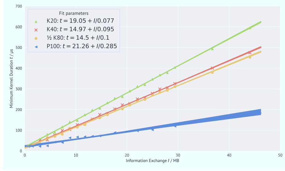
Fig. 3: GPU kernel duration as a function of exchanged information for four different GPUs: K20, K40, 1/2 K80, and P100. Shown in the legend are fit parameters to the performance model.
