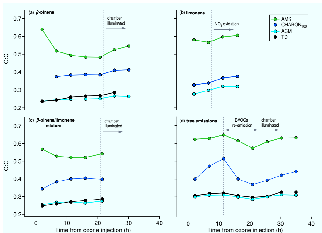
Figure 2: Bulk oxygen to carbon ratio comparison for the different instruments (CHARON 100 : blue, AMS: green, ACM: cyan, TD: black) versus the time from ozone injection. Experimental description details are provided in Table 1.
