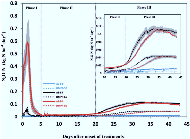
Fig. 1. Fluxes of N 2 O of soil with only mineral-N at 50% WFPS (AS-50), or mineral-N+ nitrification inhibitor at 50% WFPS (DMPP-50), or only mineral-N at 65% WFPS (AS-65), or mineral-N + nitrification inhibitor at 65% WFPS (DMPP-65), or only mineral-N at 80% WFPS (AS-80), or mineral-N + nitrification inhibitor at 80% WFPS (DMPP-80), during the 43 days of the incubation experiment. Error bars show the standard error of the mean of each treatment (n = 3).
