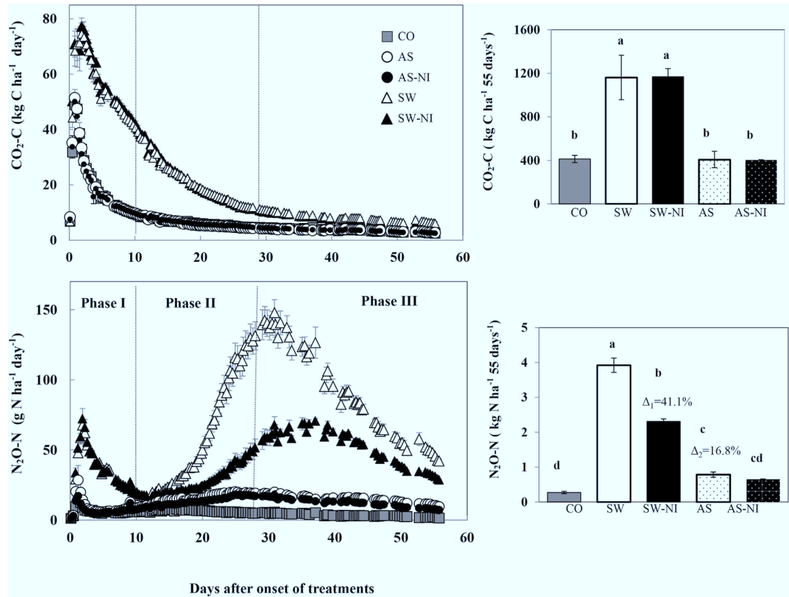
Fig. 1. Time course of fluxes and cumulative emissions of CO_2 and N_2O of soil left unamended (CO), after application of mineral-N only (AS), mineral-N + nitrification inhibitor (AS-NI), mineral-N + straw (SW) or mineral-N + straw + NI (SW-NI), during the 56 days of the incubation experiment at 70% WHC. Error bars show the standard error of the mean of each treatment ( n = 3 ). In some cases error bars are smaller than the symbols. Different lowercase letters indicate significant differences at the p < 0.05 level between treatments.
