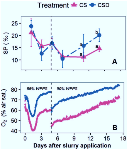
Fig. 4. (A) The corrected site preference values (SP) of soil emitted N 2 O during incubation of slurry-amended soil, and (B) average oxygen content (% air saturation) in amended soils; the vertical dashed line indicates the time of the simulated rain event of 1.25 mm precipitation following gas sampling on day 5. Error bars present standard deviation of the SP mean ( n = 4) and different letters indicate significant differences between the mean SP values of the CS and CSD treatments on each sampling day with P < 0.05.
