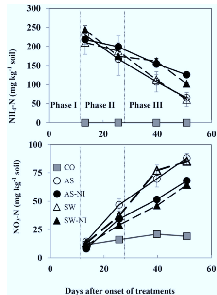
Fig. 2. Time course of \text{NH}_4^+ (mg \text{NH}_4^+-\text{N} kg ^{-1} dry soil) and \text{NO}_3^- (mg \text{NO}_3^--\text{N} kg ^{-1} dry soil) concentration of soil left unamended (CO), after application of mineral-N only (AS), mineral-N + nitrification inhibitor (AS-NI), mineral-N + straw (SW) or mineral-N + straw + NI (SW-NI), during the 56 days of the incubation experiment at 70% WHC. Error bars show the standard error of the mean of each treatment ( n = 3 ). In some cases error bars are smaller than the symbols.
