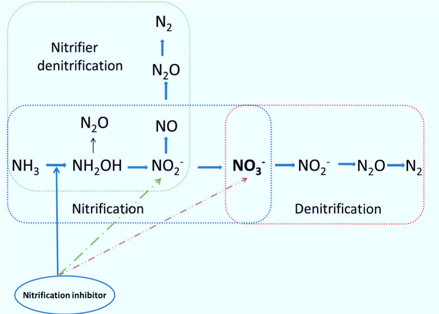
Figure 4. The direct (solid arrow) and indirect effects (dash-dot arrows) of nitrification inhibitors on N 2 O production and consumption pathways in soils.
