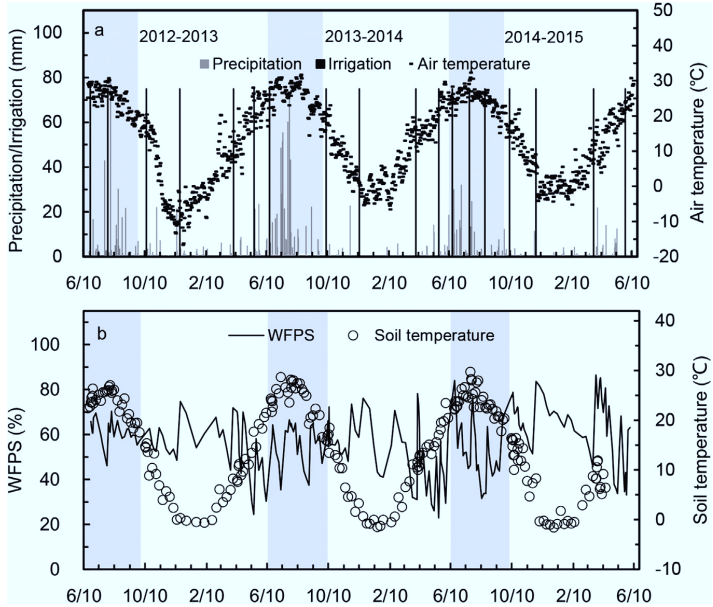
Fig. 1. Temporal variations of (a) precipitation, irrigation and air temperature and (b) soil temperature and water-filled pore space (WFPS) at the time of N 2 O sampling over the experimental period. Soil temperature and WFPS values are the means of four plot replicates. Grey background represents the maize season.
