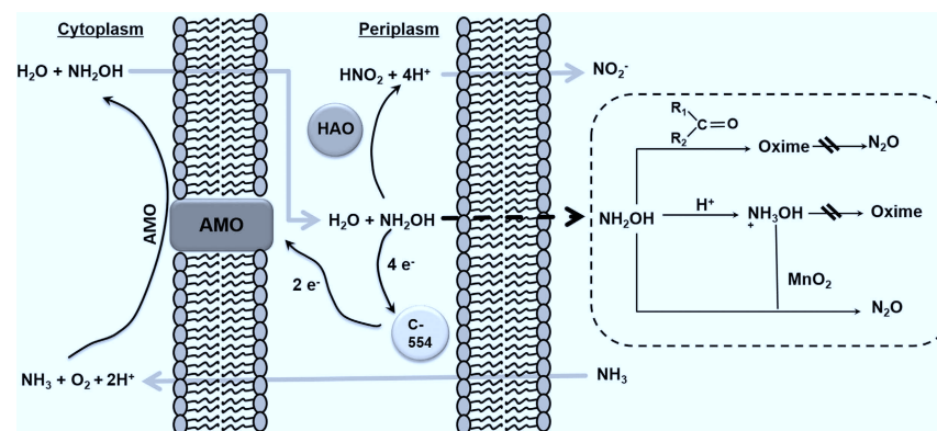
Figure 1. Hypothetical model of \text{NH}_2\text{OH} release by ammonia-oxidizing bacteria to the soil environment and potential abiotic reactions of \text{NH}_2\text{OH} with \text{MnO}_2 and organic matter in the soil at different pH conditions ( \text{R}_1\text{R}_2\text{C}=\text{O} represents carbonyl groups of SOM). AMO is ammonia monooxygenase; HAO is hydroxylamine oxidoreductase.
