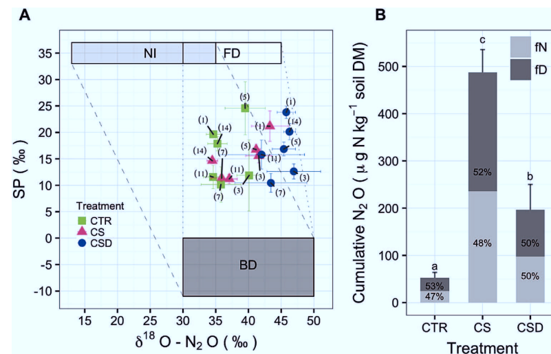
Fig. 5. (A) The end-member map with site preference values (SP) as a function of soil derived \delta^{18}\text{O-N}_2\text{O} (expressed with respect to Vienna Standard Mean Ocean Water - VSMOW) illustrates the trend shifting in source of \text{N}_2\text{O} production for the different treatments (control \blacksquare CTR, cattle slurry \blacktriangle CS and cattle slurry with DMPP treatment \bullet CSD), numbers in brackets indicate sampling days. The rectangles represent the areas corresponding to the ranges of literature data of \text{N}_2\text{O} isotopic signatures for the pure culture and soil incubation studies. SP for bacterial nitrification (NI), fungal denitrification (FD) and bacterial denitrification (BD) was based on literature data (see the method and methodology section). (B) Total cumulative \text{N}_2\text{O} over 18 days of incubation with the estimates of \text{N}_2\text{O} proportion (%) derived from NI/FD (fN) and BD (fD) based on the two-end-member mixing model. Bars indicate the standard deviation of the means ( n = 4 ).
