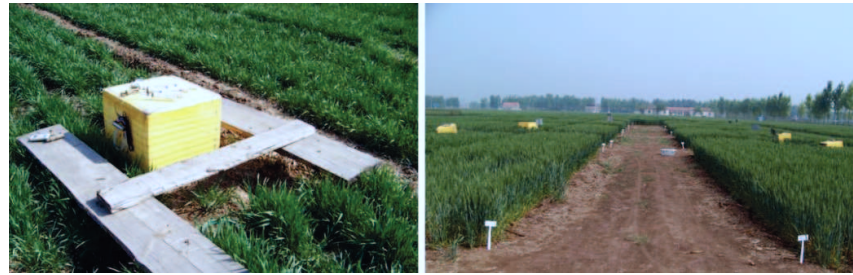
Figure 2. Static chamber used in field experiments described in Paper IV and VIII.
