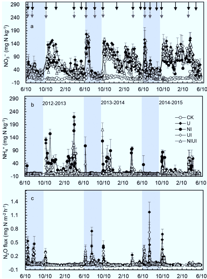
Fig. 2. (a) Soil NO 3 - content and (b) soil NH 4 + content at the time of N 2 O sampling, and (c) soil N 2 O flux over the experimental period. Data are the means ± the standard error (n = 4). Solid and dashed line arrows indicate the timing of irrigation and fertilizer application, respectively. Grey background represents the maize season.
