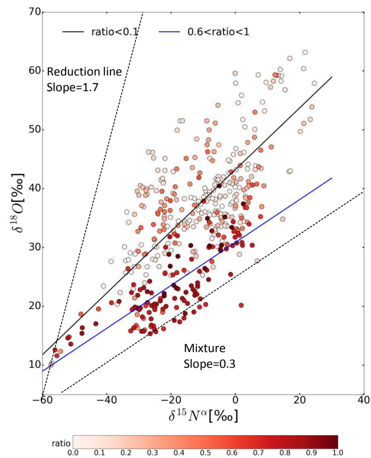
Figure 1. \delta^{18}\text{O} versus \delta^{15}\text{N}^a at different \text{N}_2\text{O}/\text{N}_2\text{O}+\text{N}_2 ratio.
