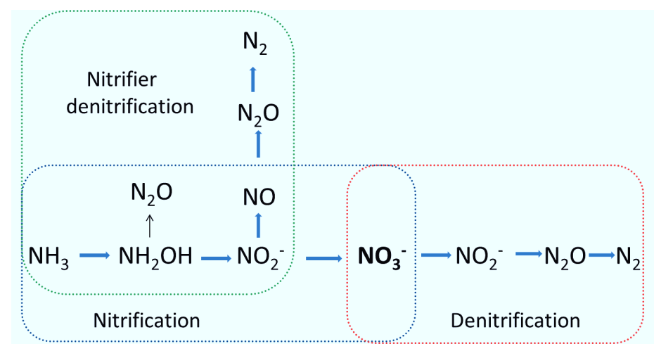
Figure 1. Three major microbial metabolic pathways that are involved in \text{N}_2\text{O} formation and consumption.
