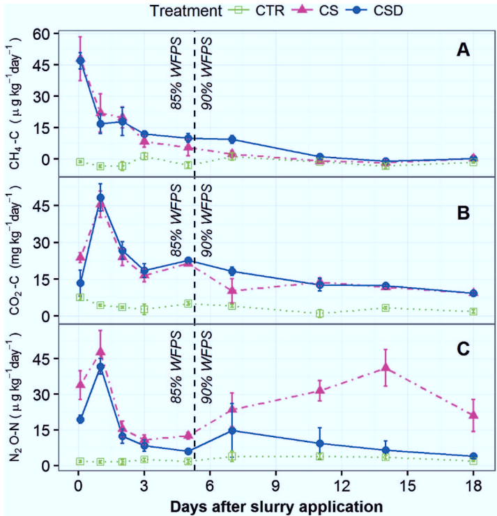
Fig. 3. Gas emission rates of CH 4 , CO 2 and N 2 O during 18 days of incubation ( n = 4, mean ± standard deviation). The vertical dashed line indicates the time of water addition. Bars indicate the standard deviation of the mean ( n = 4).
