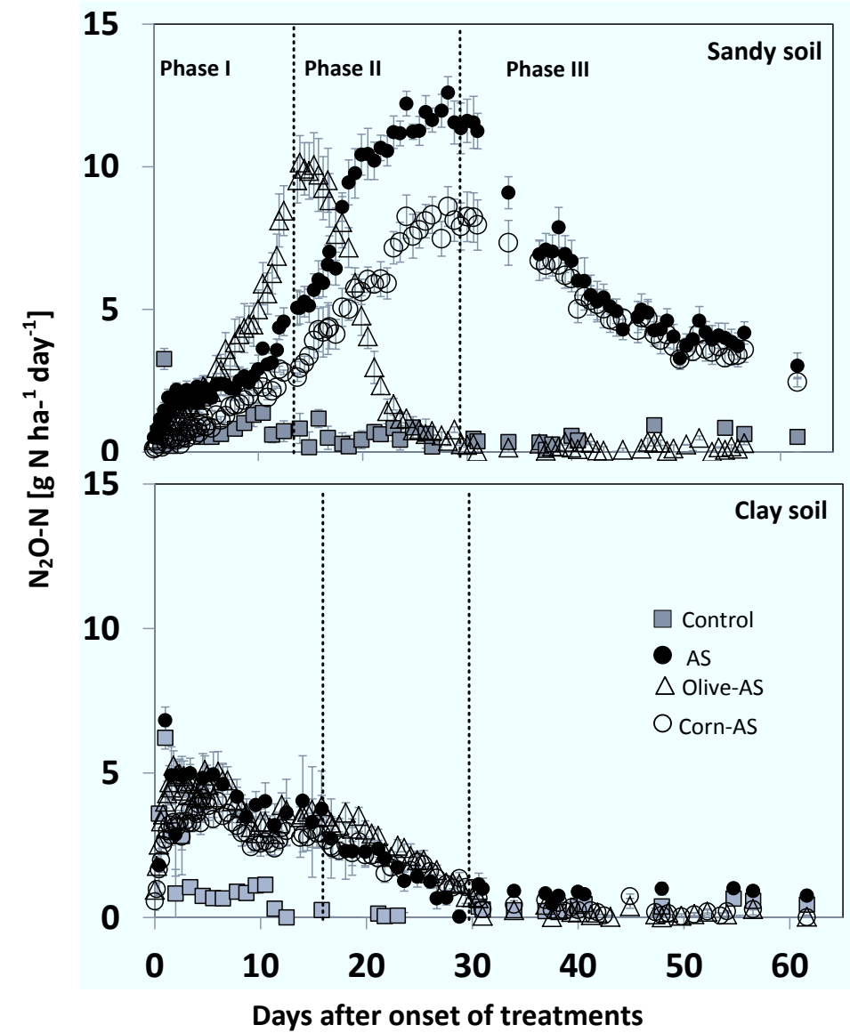
Figure 3. \text{N}_2\text{O} fluxes in the four treatments from sandy soil and clay soil. Data presented are the average of soil cores. Error bars show the standard error of the mean of each treatment ( n = 3 ).
