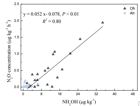
Figure 3.5 Correlation between soil \text{NH}_2\text{OH} content and aerobic \text{N}_2\text{O} emission rates at room temperature of soil samples collected from Wüstebach forest ( n = 44 ).
