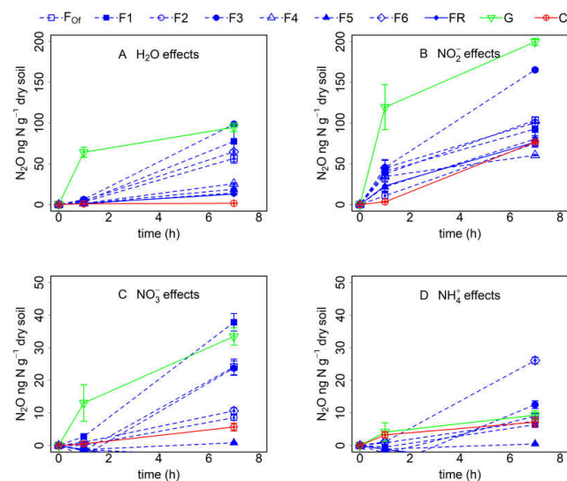
Figure 7.2 Rewetting effects by the addition of water (A), and aqueous solutions of NO 2 - (B), NO 3 - (C) and NH 4 + (D) on soil N 2 O production (ng N g -1 dry soil) of forest (F 0f , F 1 , F 2 , F 3 , F 4 , F 5 , F 6 and FR), grassland (G) and cropland (C) soil samples for different (1 and 7 h) incubation times. The values are present as mean ± standard deviation (SD).
