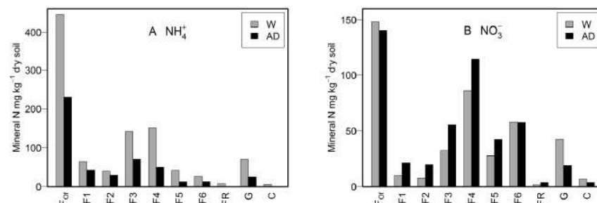
Figure 7.1 Soil \text{NH}_4^+ (A) and \text{NO}_3^- (B) content before (W, grey) and after air-drying (AD, black) for forest (For, F1, F2, F3, F4, F5, F6 and FR), grassland (G) and cropland (C) soil samples. Only one extraction was performed for the determination of soil \text{NH}_4^+ and \text{NO}_3^- content.
