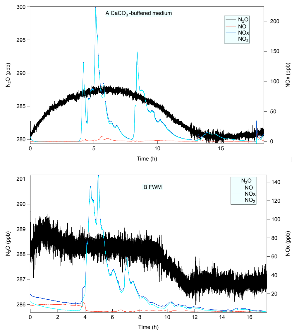
Figure S2.2 Mixing ratios (ppb) of N_2O (left y-axis) and NO_x (right y-axis) during NH_2OH (0.08 mM) abiotic decay at 37°C using an infrared laser absorption spectrometer for online real-time analysis of N_2O mixing ratio and a chemoluminescence NO_x analyzer.
