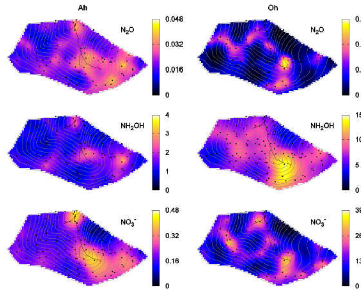
Figure 4.3 Spatial patterns of potential N 2 O emission rates ( \mu\text{g}^{-1} \text{N kg}^{-1} \text{ dry soil h}^{-1} ), NH 2 OH content ( \mu\text{g}^{-1} \text{N kg}^{-1} \text{ dry soil} ) and NO 3 - content ( \text{mg N kg}^{-1} \text{ dry soil} ) estimated using ordinary Kriging (OK) for the Ah and Oh layers of the sampling area. The grey smooth lines in the maps are contour lines. The black line represents the Wüstebach creek. The black points indicate the sampling points with valid data for each soil property.
