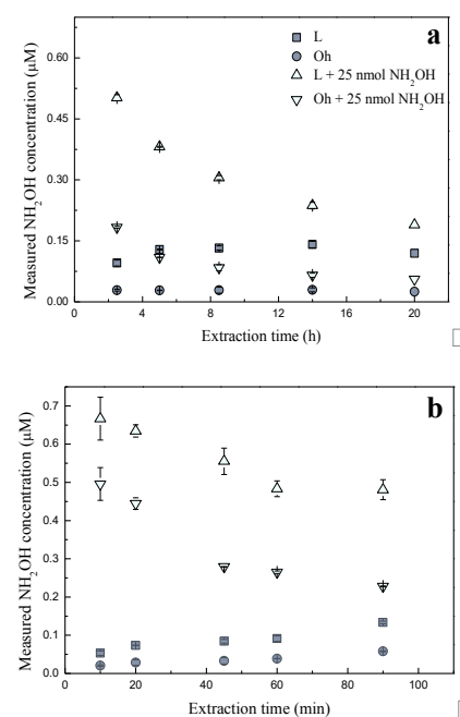
Figure 3.2 Effects of extraction time on \text{NH}_2\text{OH} concentration of the extract with shaking (a) and magnetic stirring (b) at 4 °C. Error bars indicate the range of measured concentrations (n = 2).
