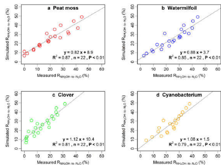
Figure 5.5 Results of the application of the artificial soil regression model for the NH 2 OH-to-N 2 O conversion ratios ( R_{\text{NH}_2\text{OH-to-N}_2\text{O}} ) to artificial soil mixtures amended with the different organic materials ( n=22 ). The three points for which R_{\text{NH}_2\text{OH-to-N}_2\text{O}} was determined at pH 3, 4, and 5 without MnO 2 addition were excluded for a better simulation.
