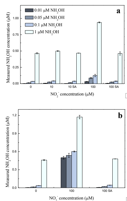
Figure 3.3 Effect of 10 and 100 \mu\text{M} \text{NO}_2^- on \text{NH}_2\text{OH} conversion with and without sulfanilamide (SA) in 0.05 M acetic acid + 0.01 M HCl solution (a) and soil extracts (b) at pH 2 and room temperature. Error bars indicate the standard deviation of the mean ( n = 3 ).
