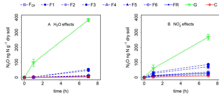
Figure 7.3 Rewetting effects by the addition of water (A) and aqueous \text{NO}_2^- (B) solution on soil \text{N}_2\text{O} production ( \text{ng N g}^{-1} dry soil) of forest ( \text{F}_{\text{Or}} , F1, F2, F3, F4, F5, F6 and FR), grassland (G) and cropland (C) soil samples for different (1 and 7 h) incubation times after \gamma -irradiation. The values are present as mean \pm standard deviation (SD).
