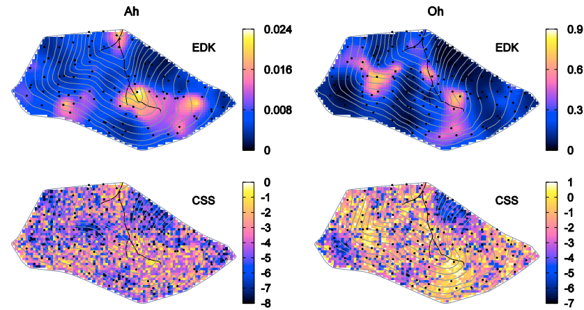
Figure 4.4 Spatial patterns of potential N 2 O emission rates estimated using external-drift Kriging (EDK) and conditional stochastic simulations (CSS) for the Ah and Oh layers. The EDK estimation is an extension of ordinary Kriging (OK) by using spatial regression estimates based on the regression models as auxiliary data. The CSS estimation is an estimation based on the spatial variability and spatial structure by checking the cumulative probability density function. The color code of the EDK maps represents N 2 O emission rates in \mu\text{g}^{-1} \text{N kg}^{-1} \text{dry soil h}^{-1} , while the color code of the CSS maps represents the logarithm of N 2 O emission rates in \mu\text{g}^{-1} \text{N kg}^{-1} \text{dry soil h}^{-1} .
