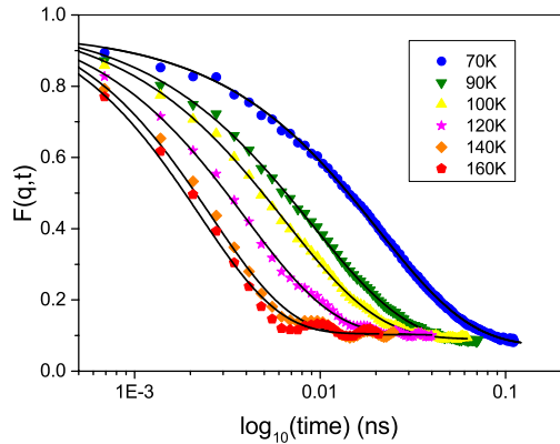
FIG. 6. Fourier transformed quasielastic data and their fit with a stretched exponential function (line) at different temperatures
