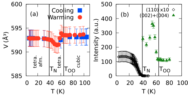
FIG. 2. (a) Temperature-dependent change of the unit cell volume V as determined using neutron diffraction. Note that the error bars include the instrument resolution as systematic error. (b) The intensities of the \vec{Q} = (110) and the \vec{Q} = (004) Bragg reflections as a function of temperature illustrating the structural transition at T_{OO} = 63 K and magnetic ordering temperature of T_N = 42 K. The data in (b) was taken using the RITA spectrometer in two-axis mode with E_i = 5 meV. The (004) Bragg peak was measured at the (002) position using \lambda/2 with the scattered Be filter removed. Note that the intensity of (110) has been magnified by a factor of 10 relative to the (004) data.
