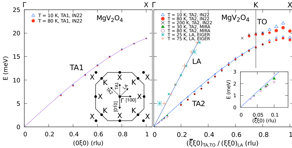
FIG. 4. The dispersion of the TA1 and the LA modes is independent of T when going from the tetragonal to the cubic phase. When comparing the cubic ( T > 63 K) to the tetragonal ( T < 63 K) phonon branches, the TA2 modes show a spoonlike behavior at intermediate q values. The sizes of the symbols indicate the sizes of the error bars. The inset in the left panel shows the hk0 plane of the face-centered cubic Brillouin zone and the scan directions. The inset in the right panel shows a magnification of the low- q TA2 phonon branch.
