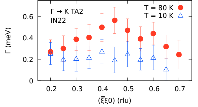
FIG. 6. Linewidth \Gamma_p of the TA2 phonon branch. In the tetragonal phase at 10 K (blue triangles), \Gamma_p is independent of momentum transfer. In the cubic phase at T = 80 K (red points), \Gamma_p attains a maximum halfway from the \Gamma to the K point.
