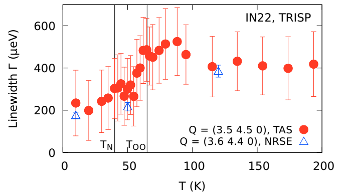
FIG. 7. Temperature dependence of the TA2 phonons at Q = (3.5 \ 4.5 \ 0) using conventional TAS spectroscopy (red dots) and Q = (3.6 \ 4.4 \ 0) using TRISP (blue triangles). A subtle plateau can be identified between T_N and T_{OO} . \Gamma_p increases to approximately 0.45 meV in the cubic phase where it remains constant up to T = 200 K.
