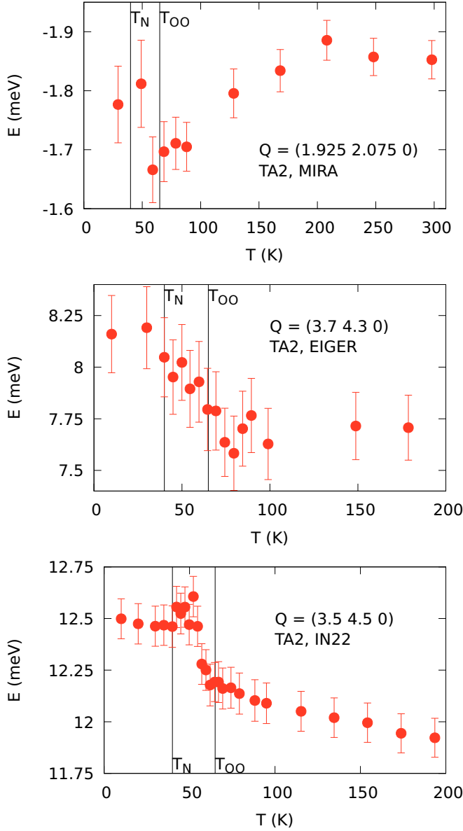
FIG. 5. The dispersion of the TA2 phonons softens and hardens at q = (0.075 \ 0.075 \ 0) (top) and q = (0.5 \ 0.5 \ 0) (bottom), respectively, when approaching the cubic-tetragonal phase transition near T_{OO} = 63 K from high temperatures. For q = (0.3 \ 0.3 \ 0) (middle) there is no change in phonon energies in the T > T_{OO} region. Please note that at MIRA we measured using neutron energy gain ( -E ) for reasons of analyzer efficiency and angular constraints at the instrument. The physics of the system is unaffected by this choice.
