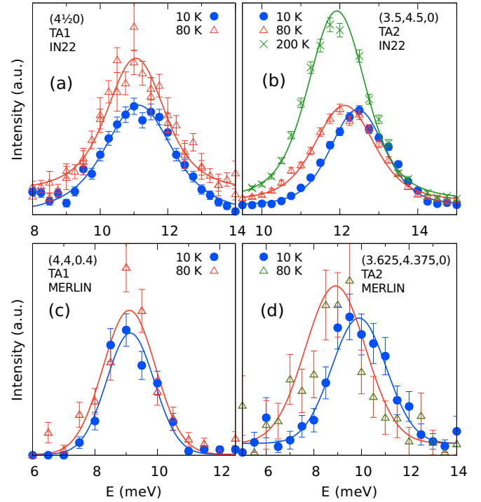
FIG. 3. Typical data for transverse phonons TA1 and TA2 are shown for T = 10 K and T = 80 K. There is a clear softening of the TA2 mode in the cubic phase when compared with the low temperature tetragonal phase.
