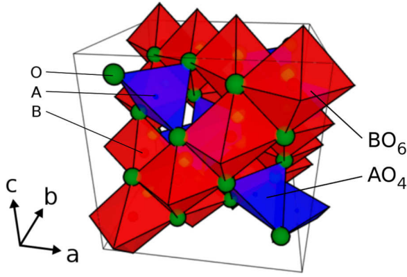
FIG. 1. Conventional unit cell of a spinel. In an AB_2O_4 spinel, the A metal ions are in a tetrahedral AO_4 environment that constitutes a diamond lattice, and the B metal ions form edge-sharing BO_6 octahedra arranged in a pyrochlore lattice.
