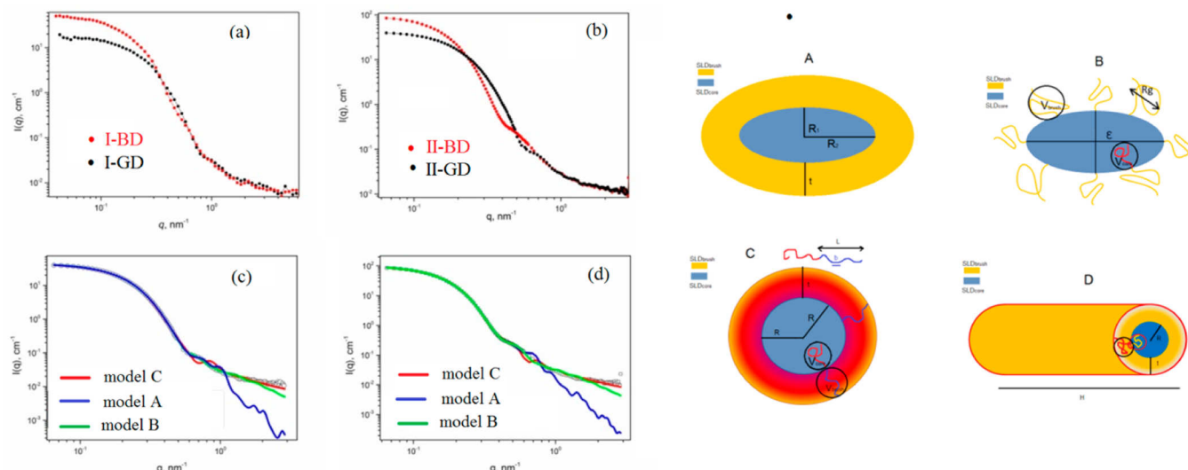
Figure 1. SANS data for (a) I-GD and I-BD in D 2 O (solvent 2, Table S3); (b) II-GD and II-BD in D 2 O (solvent 2, Table S3). (c) II-GD in 40% d 6 -EtOH+60% D 2 O (solvent 10) with different fits; (d) II-BD in 40% d 6 -EtOH+60% D 2 O (solvent 10) with different fits. Scattering curves were extrapolated to infinite dilution. The models for SAXS and SANS data fitting; (A) core–shell ellipsoid, (B) elliptical block copolymer micelle with random walk chains, (C) spherical micelle with homogeneous core and radial decaying density shell with self-avoiding chains, and (D) rod-like micelle with rod-like homogeneous core and radial decaying density shell.
