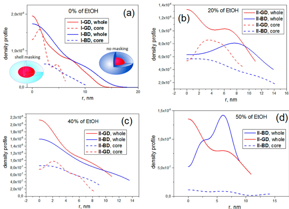
Figure 2. Contrast density profiles obtained by deconvolution of the PDDF shown in Figure S11c,d. (a) 0% of EtOH; (b) 20% of EtOH; (c) 40% of EtOH; (d) 50% of EtOH.
