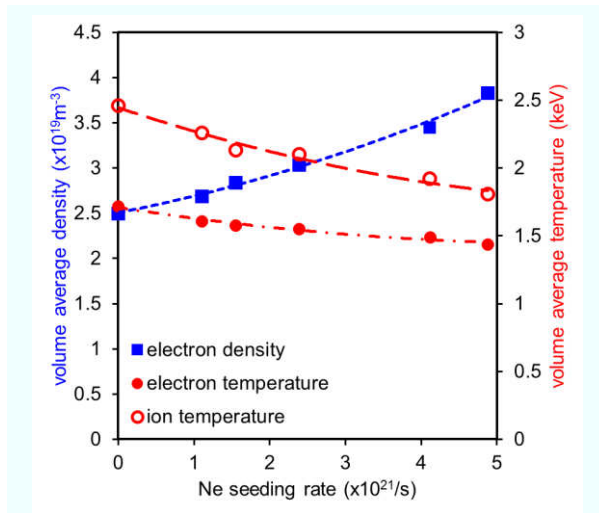
Fig.3 Plasma density and temperature during analysis time window ( t_{NBI}+1.70 to t_{NBI}+1.95 s) versus Ne seeding rate (in electrons/s averaged during t_{NBI}-0.3 s to t_{NBI}+1.7 s).
