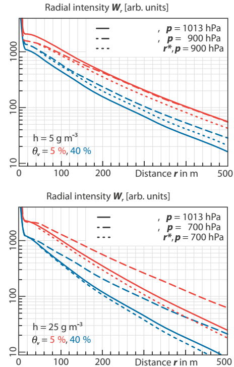
Figure A1. Pressure dependence of the weighting function W_r , demonstrated for two cases of air pressure and humidity. The rescaled p -adapted curves (dots, Eq. A1) are almost parallel to the non-adapted curves (solid), indicating that the normlized weight leads to the same results. (a) Dry midlands; (b) humid highlands.
