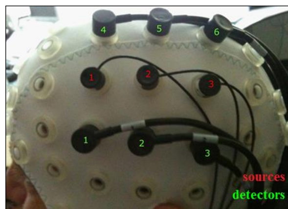
Figure 2: fNIRS optode set-up with the source optodes in red (optodes 1, 2 and 3 in the middle horizontal line) and detector optodes 1-6 in green.
