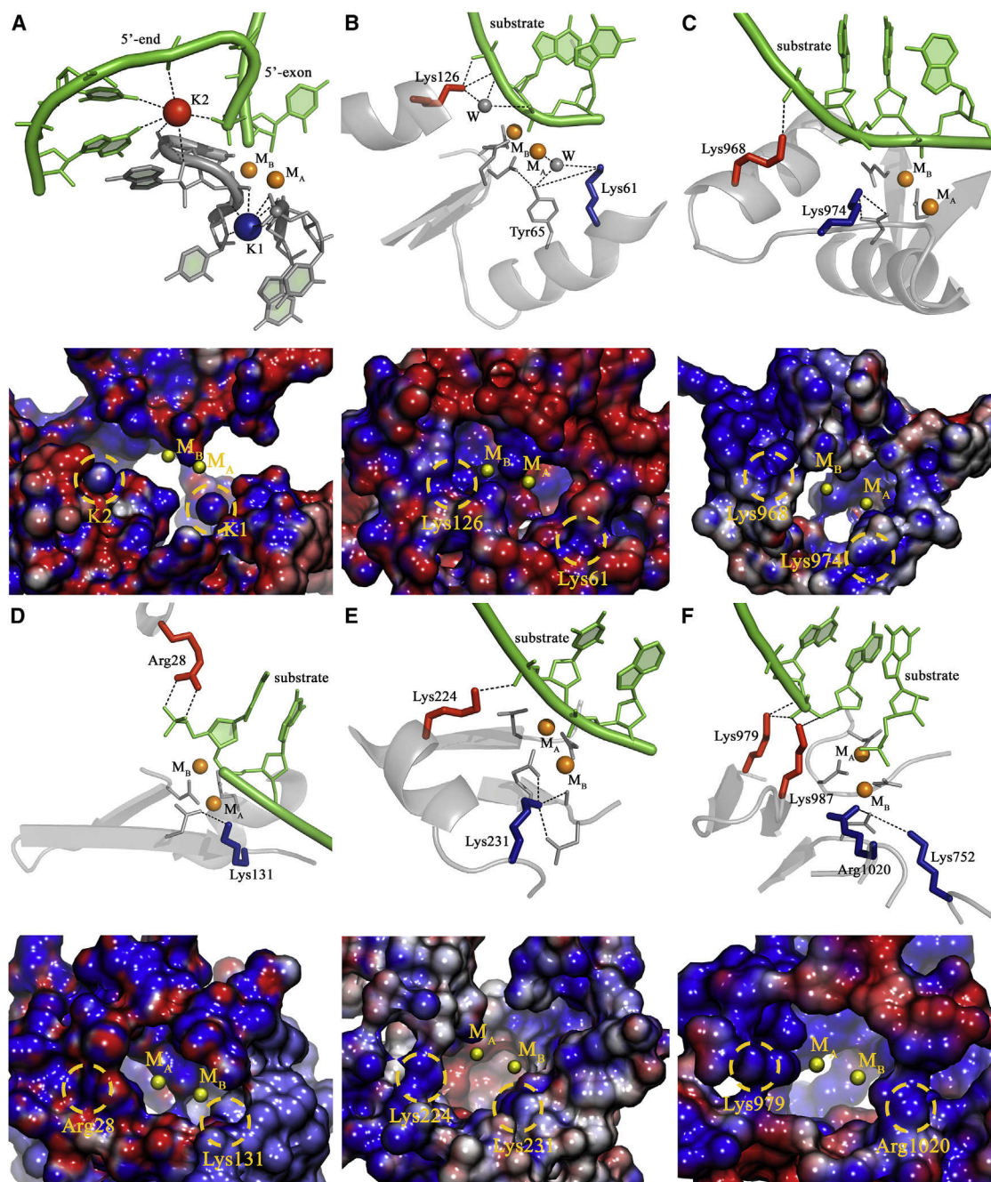
Figure 1. Structural Comparison of the Catalytic Sites of Representative Two-Metal-Ion Enzymes
