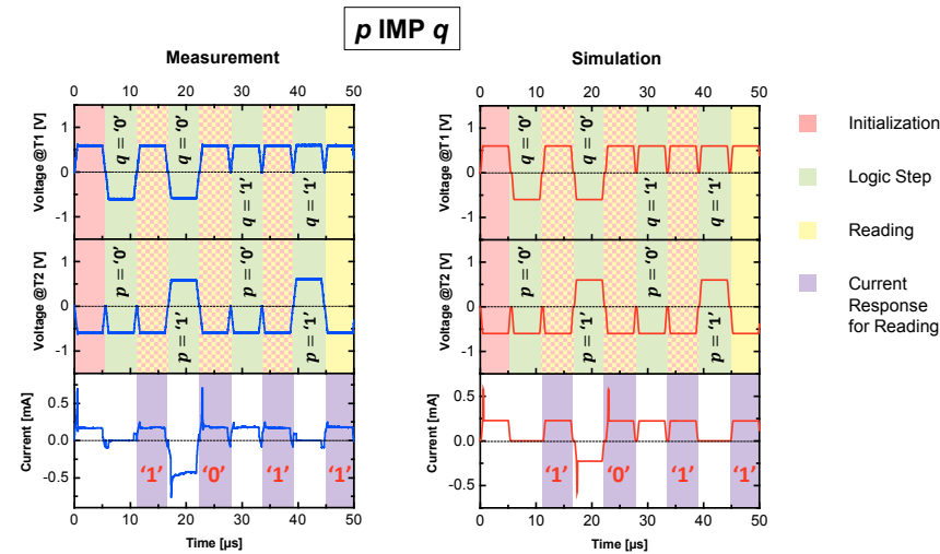
Figure 7.23: Measurement (left) and simulation (right) of the logic IMP function by two steps for the nano-BC CRS under pulse conditions. Simulations have been performed by A. Siemon.[4] (Redrawn with permission from the publisher.)
