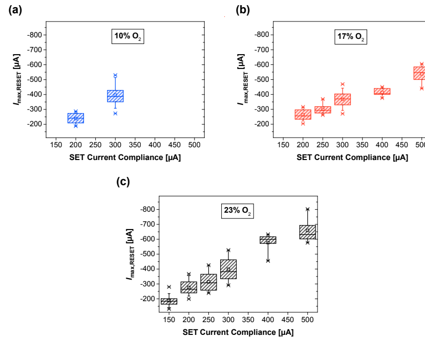
Figure 5.10: Maximal RESET current as function of applied current compliance for SET process. Independent of the relative \text{O}_2 sputtering gas flow for the \text{HfO}_2 deposition, all devices follow the same trend.
