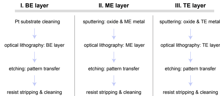
Figure 4.11: Flowchart for the three-terminal micro-BC CRS device, referred to as structure A. The complete process requires three processing steps: bottom electrode (BE), middle electrode (ME) and top electrode (TE) layer patterning.
