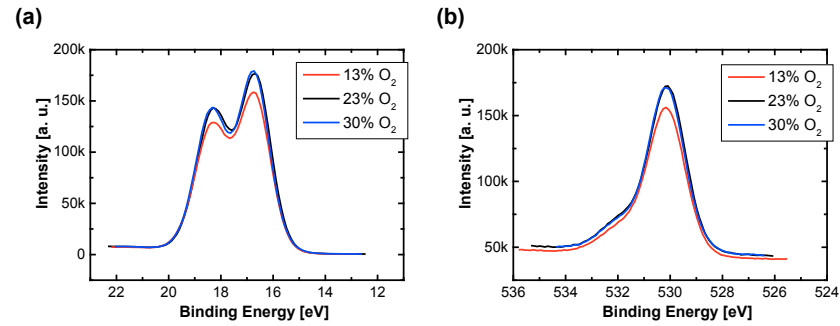
Figure 4.4: XPS of as-deposited HfO 2 for different relative O 2 sputtering gas flow. (a) Hf-4f spectra and (b) O-1s spectra. The variation of relative O 2 sputtering gas flow does not change the composition ratio of Hf and O. (With kind approval of A. Besmehn, ZEA-3, FZ Jülich)
