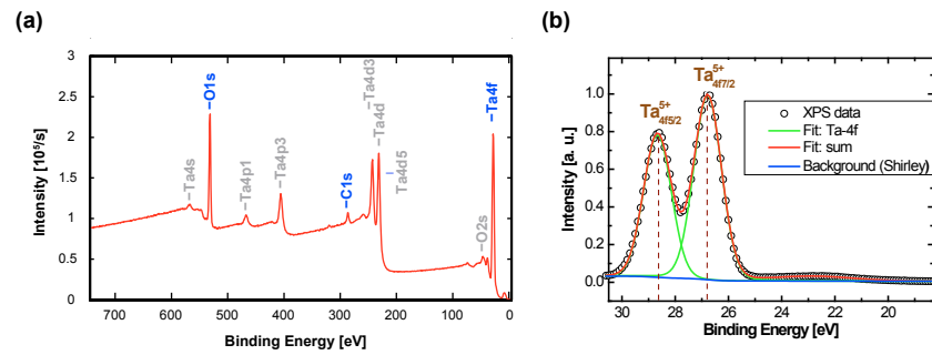
Figure 4.5: XPS of as-deposited Ta 2 O 5 . (a) Survey scan with highlighted core levels (blue labeled), which are further investigated. (b) Detailed scan of the Ta-4f peak, which is split into a doublet. (With kind approval of A. Besmehn, ZEA-3, FZ Jülich)
