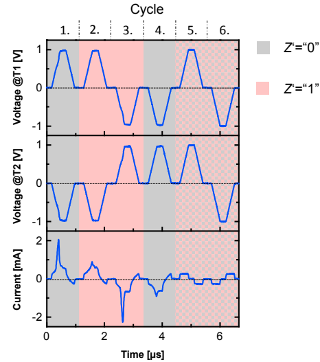
Figure 7.9: Feasible pulsed voltage / state configurations of the CS device with related transient current response. The difference of potentials applied to the terminals T1 and T2 determines the overall voltage drop ( V_{\text{tot}} = V_{T1} - V_{T2} ). Z' is the CS state before applying signals to T1 and T2, with Z' = '0' (gray) or Z' = '1' (rose). If the signals are equal, only (dis-)charging current is observed (independent of Z' ). For all configurations, the transient current responses are unique. Consider, the switching current depends on the electroforming procedure and the applied pulse parameters. For example, steep rising and falling ramps of voltage pulses result in larger current levels (in comparison to quasi-static experiments), since the CS is not able to respond quasi-statically to the voltage drop. Rather, it shows an instantaneous switching via the 'ON' transition state, causing the typical current spike.[2] (Reprinted with permission from the publisher.)
