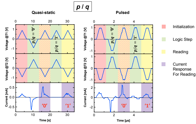
Figure 7.12: The CRS-logic p/q function performed by two steps under quasi-static and pulse conditions. It should be noted this logic operation depends only on one input variable (either p or q ) and overall only two input configurations are available.[2] (Reprinted with permission from the publisher.)
