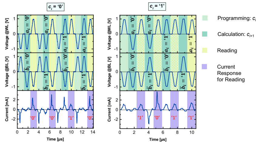
Figure 7.27: Implementation of the carry as defined by Equation 7.4. c_{i+1} depends on the inputs ( a_i and b_i ) and the previous carry ( c_i ): c_i = '0' (left) or c_i = '1' (right). Background colors of the graph highlight the different operations. Reading results are displayed by red lettering.[2] (Reprinted with permission from the publisher.)
