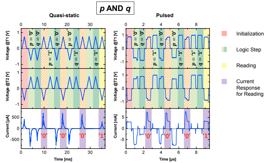
Figure 7.22: Measurement of the logic AND operation by two steps for (left) the nano-BC CRS under quasi-static conditions and (right) for the micro-BC CRS under pulse conditions.[4] (Redrawn with permission from the publisher.)
