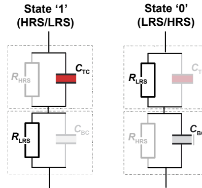
Figure A.4: Associative capacitive network (ACN) scheme. The concepts have been introduced by Tappertzhofen et al. in [136] and by Kavehei et al. in [144]. Bottom cell (BC) and top cell (TC) distinguish in capacitance for the individual high resistance state. Therefore, total device capacitance is different for the two CRS states ('1' and '0' or rather HRS/LRS and LRS/HRS).[144] (Redrawn with permission from the publisher.)
