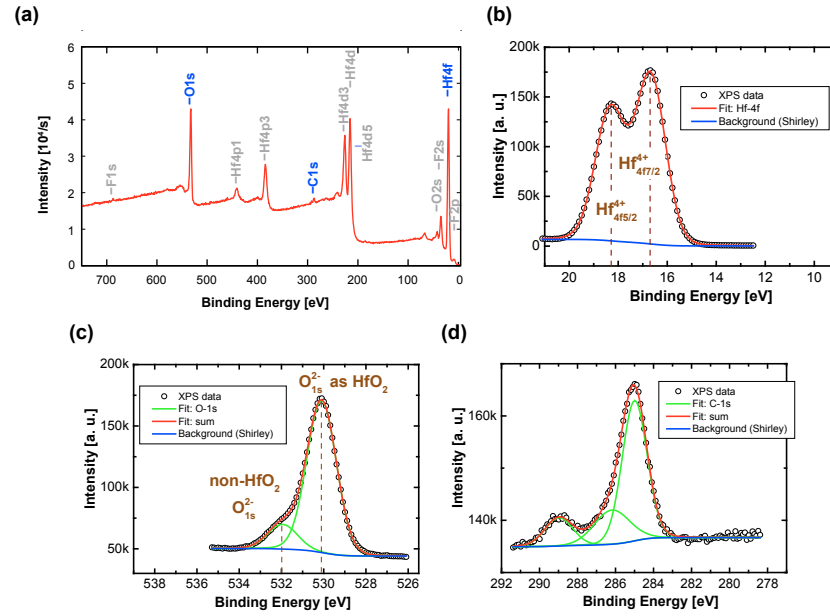
Figure 4.3: XPS analysis of as-deposited \text{HfO}_2 . (a) Survey scan with highlighted core levels (blue labeled), which are further investigated. (b) Detailed scan of the Hf-4f peak, which is split into a doublet. (c) Detailed scan of the O-1s spectrum. (d) Detailed scan of C-1s peak caused by typical surface contamination by carbon, which is used for the energy level calibration. (With kind approval of A. Besmehn, ZEA-3, FZ Jülich)
