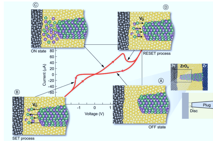
Figure 2.1: Valence Change Mechanism (VCM) switching scheme. The quasi-static I - V characteristic of a \text{Pt}|\text{ZrO}_x|\text{Zr} valence change memory. Consider, the displayed voltage is applied to the Pt electrode, whereas the Zr electrode is grounded. The sketches A to D present the switching stages. The oxygen vacancies are represented by green balls, whereas the purple ones indicate the Zr ions being in a lower valence state. (A) HRS (or ‘OFF’ state), (B) SET process, (C) LRS (or ‘ON’ state) and (D) RESET process.[48] (Reprinted with permission from the publisher.)
