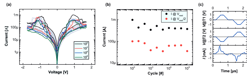
Figure 5.20: Endurance experiment of the HfO 2 -based CS. (a) I - V -characteristic for quasi-static voltage ramps after n pulsed cycles (alternating positive and negative pulses). Consider, fluctuations in the highly resistive CS states are observed (i.e. cycle 10^3 for positive polarity), which might be caused by atomistic nature of the conductive filament.[117] (b) Read selectivity extracted from the recorded endurance data (at read voltages V_{\text{read}} = 1 V and at V_{\text{read}}/2 ). (c) Transient response current after the endurance experiment.[2] (Redrawn with permission from the publisher.)
