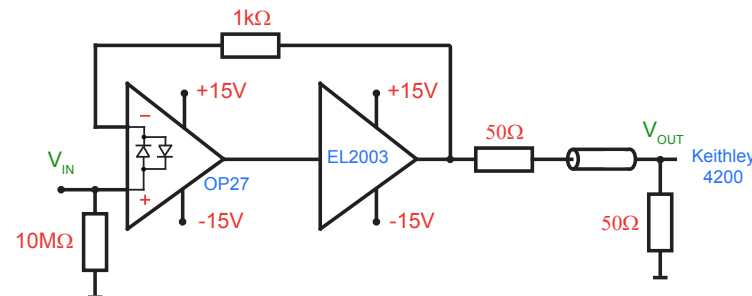
Figure 3.5: Simplified circuit of impedance converter for detecting pulse output signals in MIN / MAX gates.
