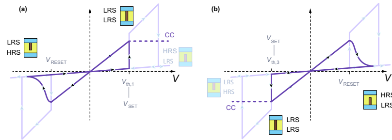
Figure 5.3: Complementary switching (CS) vs. bipolar switching (BS) in \text{HfO}_2 -based devices. BS I - V characteristic (a) in the eight-wise switching mode and (b) in the counter-eight-wise switching mode. The insets show the resistance scheme at the electrode interfaces. Switching at the second interface is suppressed by the instrument current compliance (CC). The pale curve indicates the CS I - V characteristic without CC.
