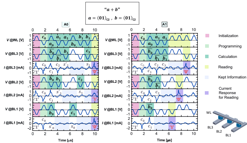
Figure 7.28: Pre-Calculation (PC) Adder: proof-of-concept experiment for the operation “ a + b ” with a = (01)_{C2} and b = (01)_{C2} , where C2 indicates the two’s complement notation. The main / auxiliary calculations are conducted in the array A0 / A1. Reading results are displayed by red labeling. Background colors of the graphs highlight the different operations. Significant bits, which are applied WLs and BLs, are pointed by black lettering. Actual stored cell information is displayed once in the current response line (gray labeling). The lower right illustration depicts the used 1 \times 3 crosspoint array with the terminals WL and BL1 to BL3 for the input signals.[2] (Reprinted with permission from the publisher.)
