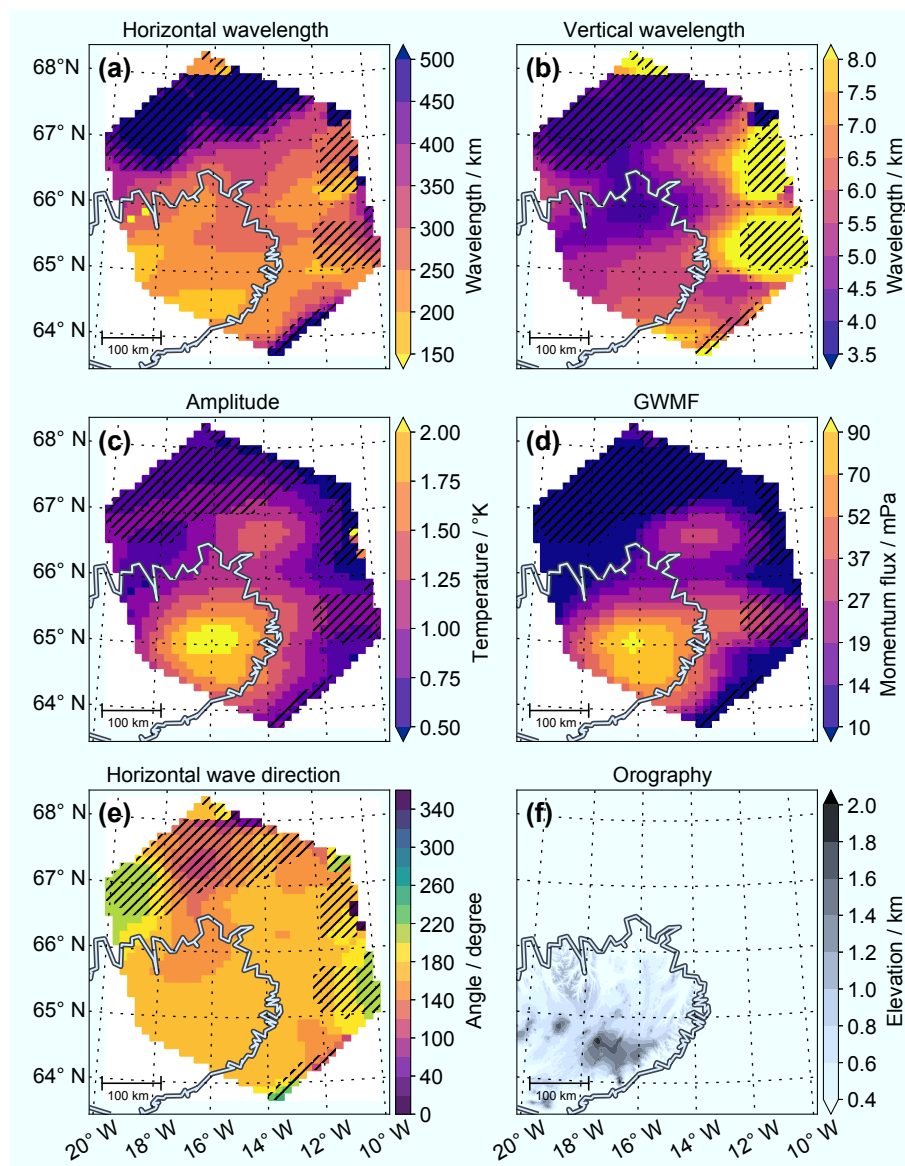
Figure 5. Three-dimensional sinusoidal wave fit of the GLORIA measurements in fitting cubes of 160\text{ km} \times 160\text{ km} \times 3.6\text{ km} at a center height of 11.5 km. Nonsignificant fitting results with wavelengths above 2.5 times the cube size are hashed. These parameters are used to drive the GROGRAT model, the results of which are shown in Fig. 7. Panel (e) shows the direction of the horizontal wave vector. Eastward direction corresponds to 90^\circ and southward direction to 180^\circ .
