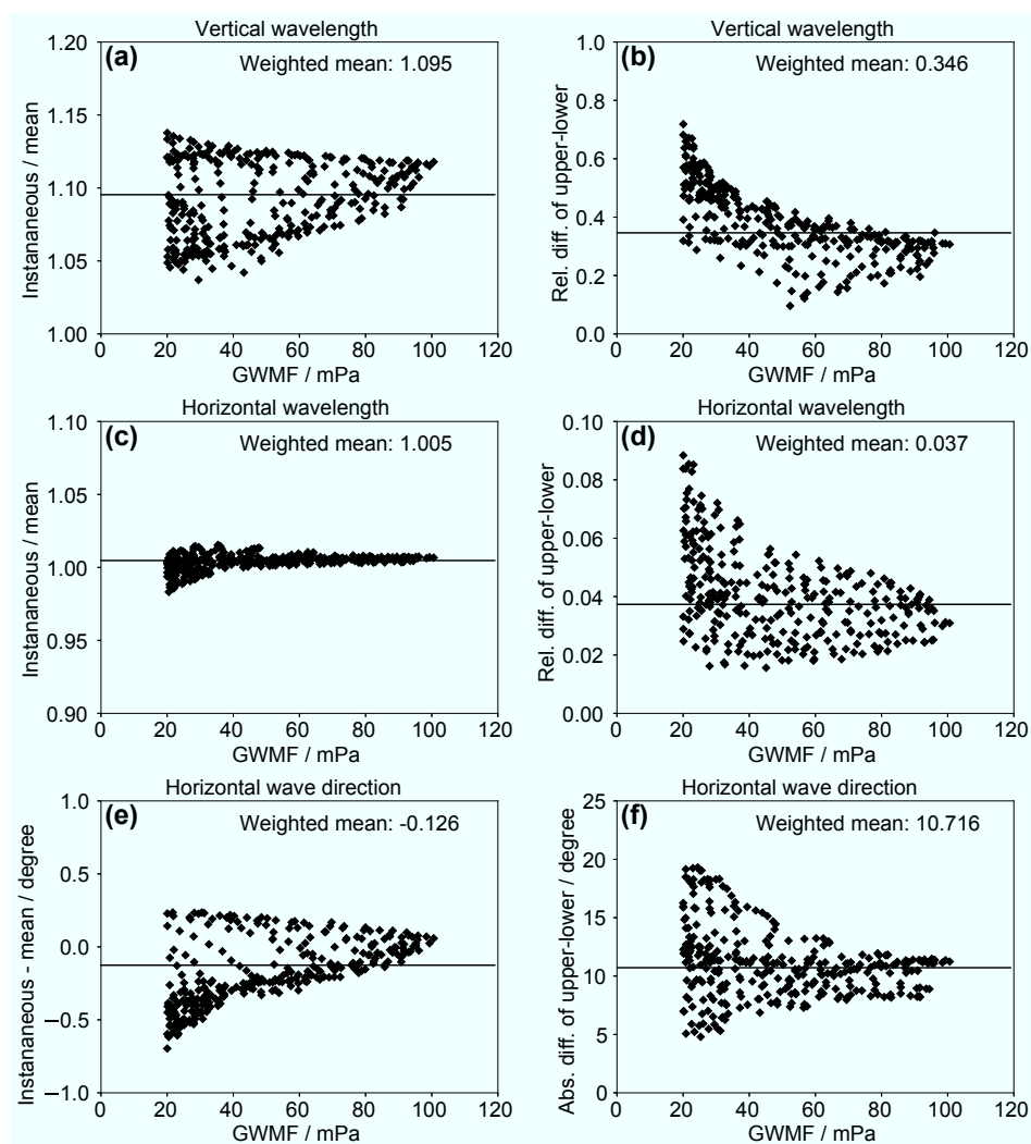
Figure A1. Comparison of mean values over the whole S3D fitting volume and instantaneous values in the middle for different wave parameters ( a , c , e ) and variation of wave parameters from the lower to the upper boundary of the S3D fitting volume ( b , d , f ). For all graphs GWMF weighted means are calculated and depicted as black lines.
