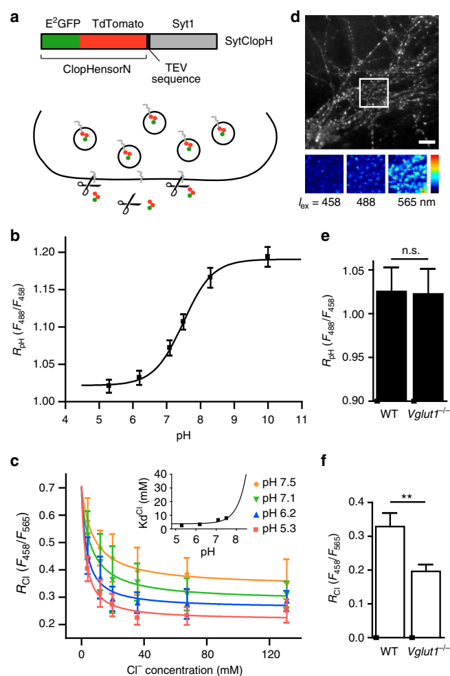
Fig. 4 Absence of VGLUT1 prevents the efflux of luminal \text{Cl}^- . a The synaptotagmin 1-ClopSensorN (SytClopH) construct is composed of the previously described ClopSensorN (E 2 GFP-TdTomato fusion) 37 fused to the cleavage site for recombinant TEV protease and synaptotagmin 1 (Syt1) (top). When neurons-overexpressing SytClopH were exposed to 60 U ml -1 TEV protease (scissors) at room temperature, ClopSensorN was cleaved from molecules residing in the plasma membrane while vesicular SytClopH was inaccessible to the protease (bottom). b SytClopH calibration curve relating pH to the ratio of fluorescence emission when E 2 GFP was excited at 488 nm over the emission when excited at 458 nm ( R_{pH} ). pKa was found to be 7.49 with a fitted 95% confidence interval between 7.23 and 7.76. Note that variation of \text{Cl}^- concentration within the physiological range had no effect on R_{pH} (Supplementary Fig. 7). c SytClopH calibration curve relating \text{Cl}^- concentration to the ratio of fluorescence emission when E 2 GFP was excited at 458 nm over the emission when TdTomato was excited at 565 nm ( R_{Cl} ). Change in pH influences the affinity of SytClopH for \text{Cl}^- . d Fluorescence image of hippocampal axonal arborisations of wild-type neurons expressing SytClopH collected following excitation at 565 nm. The insets (bottom) show a higher magnification with excitation at 458, 488 and 565 nm respectively. Scale bar represents 10 \mu\text{m} . e , f Histogram of the measured R_{pH} ( e ) and R_{Cl} ( f ) in hippocampal neurons from wild-type (WT, n=29 ) and VGLUT1 knock-out ( Vglut1^{-/-} , n=27 ) mice. n.s. not significant P=0.9447 ; ** P=0.0060 analysed with two-tailed unpaired t -test. Error bars represent s.e.m.
