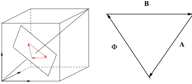
FIG. 1. Projection of the position of the directed polymer onto the plane perpendicular to the (1,1,1) direction (left) and directions for the 2D height function (right).
