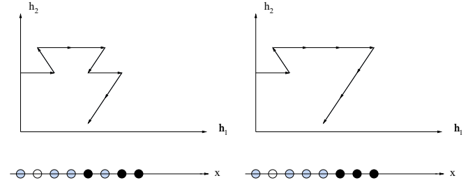
FIG. 2. Two-dimensional random path on the honeycomb lattice and diffusing particles. From the left picture to the right picture, the black particle on lattice site 5 and the gray particle on lattice site 6 have interchanged places and the path has changed accordingly.
