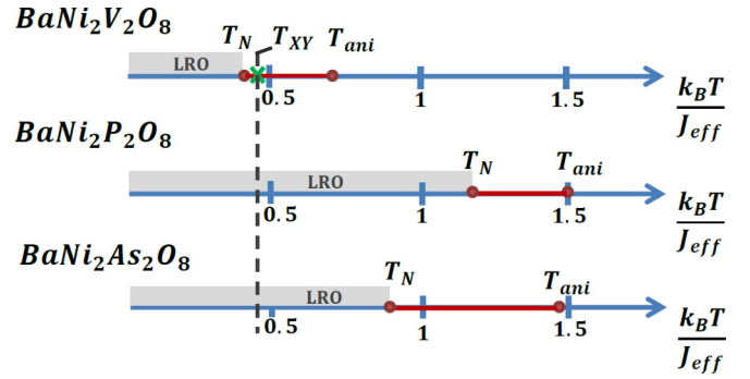
FIG. 7. The magnetic regimes of \text{BaNi}_2\text{V}_2\text{O}_8 , \text{BaNi}_2\text{P}_2\text{O}_8 , and \text{BaNi}_2\text{As}_2\text{O}_8 as a function of the relative temperature scale ( k_B T / J_{\text{eff}} ). The Néel temperature T_N and the temperature T_{\text{ani}} where the magnetic anisotropy first appears are indicated by the red filled circles. The gray area below T_N indicates the long-range magnetically ordered phase. The temperature T_{XY} , at which \chi_{H\parallel c} in \text{BaNi}_2\text{V}_2\text{O}_8 has a minimum associated with EP anisotropy regime, is marked by the green cross. The black dashed line indicates the position of T_{XY} with respect to \text{BaNi}_2\text{P}_2\text{O}_8 and \text{BaNi}_2\text{As}_2\text{O}_8 .
