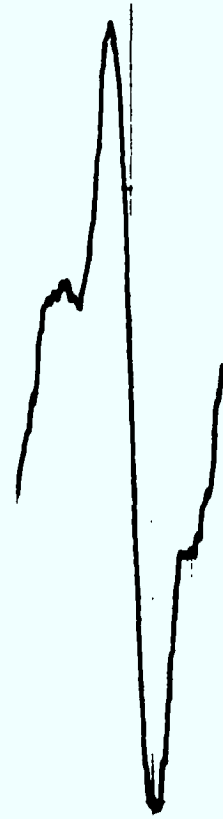
Abb. 40 SHFS in \text{SnO}_2:\text{Tc(IV)} , H \parallel [110]
