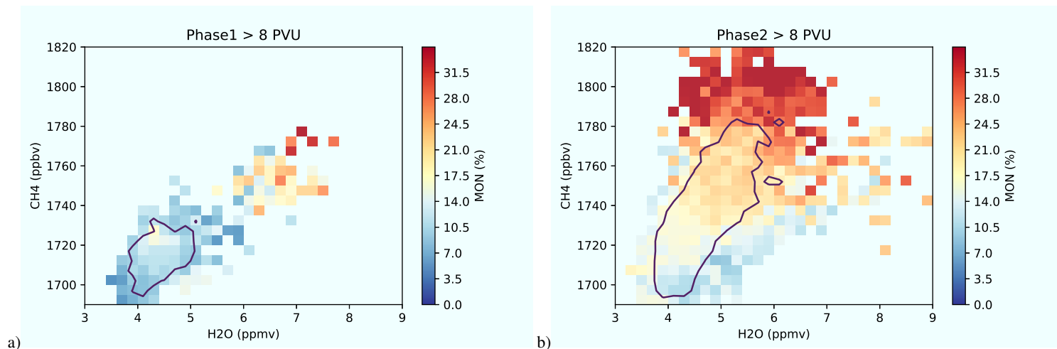
Figure 3. Correlation of water vapor and methane for PV > 8 PVU, color-coded by the Asian monsoon surface tracer MON. The solid black line represents the core region which contains 75 % of the data.
