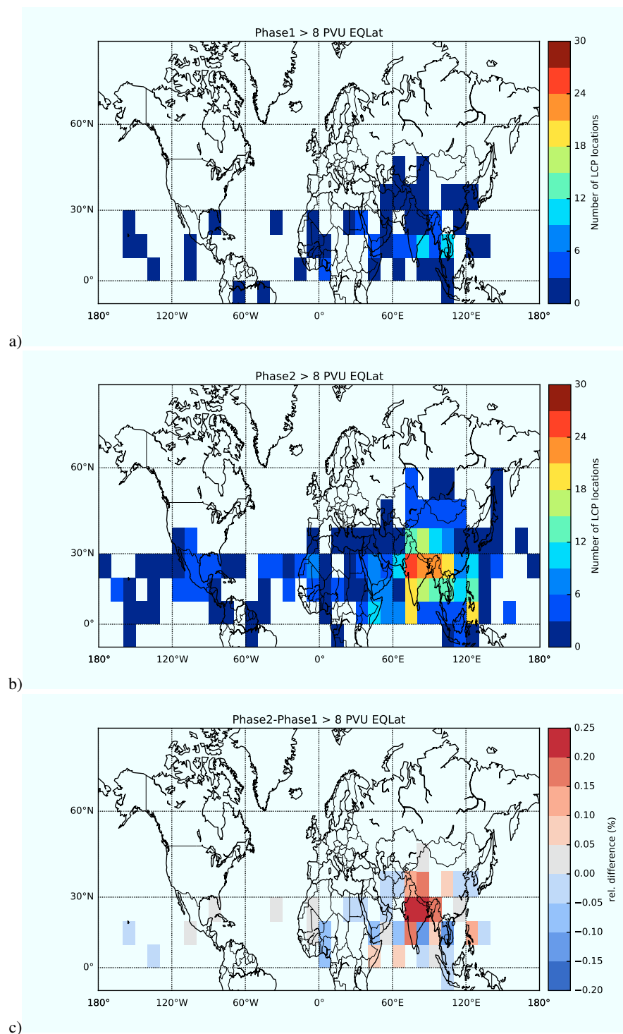
Figure 4. Location of Lagrangian Cold point (LCP) binned by longitude and latitude. LCP location for phase 1 and phase 2 are shown in a) and b), respectively. The relative difference normalized to the total number of trajectories is shown in Fig. c).
