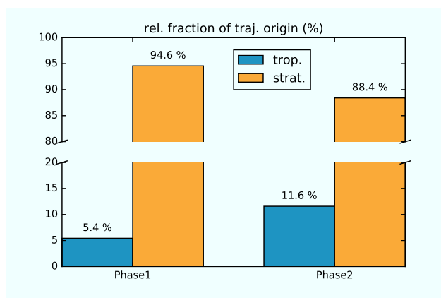
Figure 5. Fraction of trajectories with tropospheric (blue) or stratospheric (orange) origin for each phase.
