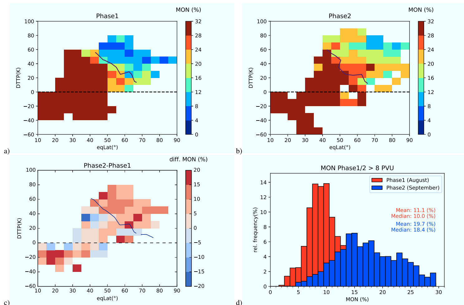
Figure 2. Same as Figure 1 but for the simulated Asian monsoon surface tracer MON.
