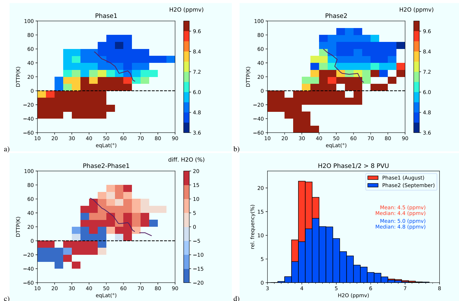
Figure 1. Mean distribution of H 2 O as a function of equivalent latitude and distance to thermal tropopause (DTTP) in potential temperature units: a) phase 1 b) and phase 2. c) Relative differences of H 2 O between phase 2 and phase 1. The dashed and the solid black line represents the thermal tropopause and the 8 PVU isoline, respectively. d) Frequency distribution of H 2 O for the lower stratosphere (PV > 8 PVU) for phase 1 (red) and phase 2 (blue). The mean and median values of each distribution given in red and blue, respectively.
