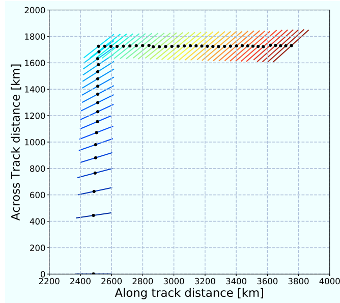
Figure 6. Illustration of the ‘sweep mode’ central measurement track. Flight direction is to the right, 0^\circ viewing direction is to the right as well. For a single measurement, the LOS that targets at 70 km tangent altitude is traced. The solid lines indicate the segments of propagation paths between 70 km and 71 km in the atmosphere. The locations of corresponding tangent points are represented by black circles.
