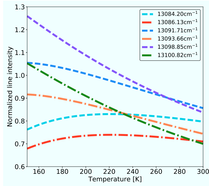
Figure 4. Temperature dependence of six rotational lines of the O 2 A-band emission. The center wavenumbers of individual lines are given in the figure legend. The intensity is normalized around the maximum intensity for a temperature of 230 K.
