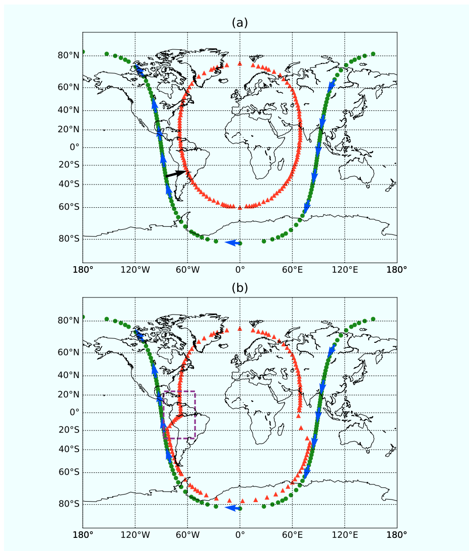
Figure 2. Global observation geometry of an exemplary orbit of (a) conventional limb sounding and (b) ‘sweep mode’ limb sounding. The satellite is operated in an orbit at an altitude of 600 km and inclination of 98^\circ . Satellite positions are sampled by green dots and corresponding tangent points by red triangles. The flight direction of the satellite is shown by blue arrows. The viewing angle in panel (a) is perpendicular to the flight direction, shown as the black arrow. In panel (b), the viewing angle changes from 10^\circ to 90^\circ in the ascending orbit, and decreases back to 10^\circ in the descending orbit.
