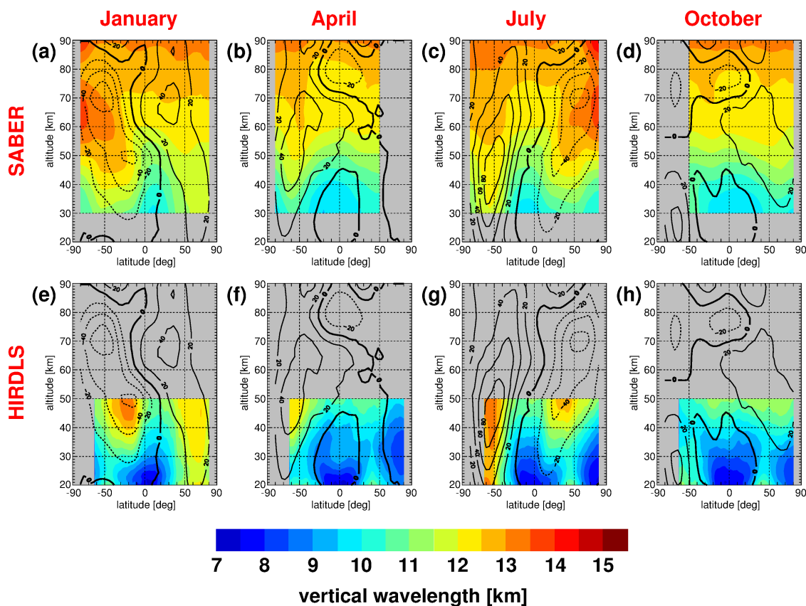
Figure 9. Latitude-altitude cross sections of zonal average gravity wave vertical wavelengths from single altitude profiles. Values are in km. Shown are multi-year averages for SABER (upper) and HIRDLS (lower) for the months of January (left column), April (second column), July (third column), and October (right column). Overplotted winds are from the SPARC climatology (Swinbank and Ortland, 2003; Randel et al., 2002, 2004). Westward (eastward) winds are indicated by dashed (solid) contour lines. The zero wind line is bold solid. Contour line increment is 20 \text{ m s}^{-1} .
