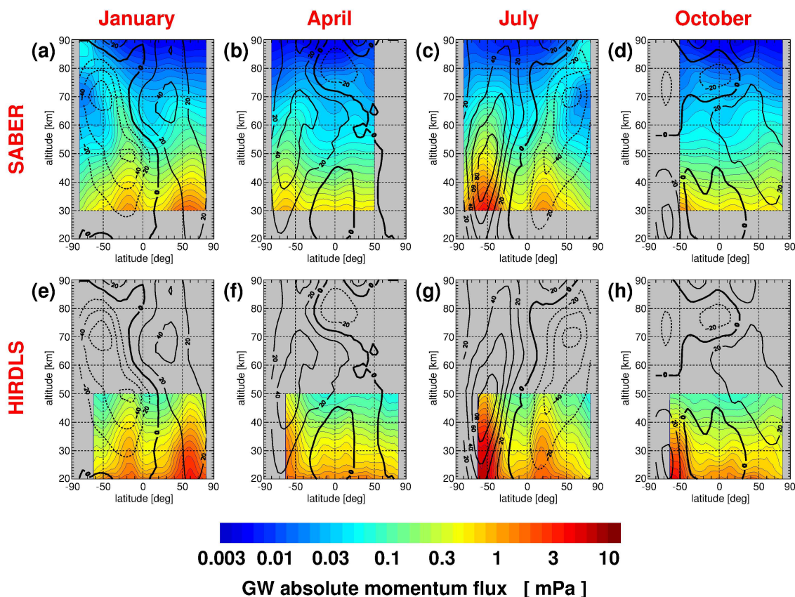
Figure 11. Latitude-altitude cross sections of zonal average gravity wave absolute momentum fluxes in mPa. Shown are multi-year averages for SABER (upper) and HIRDLS (lower) for the months of January (left column), April (second column), July (third column), and October (right column). Overplotted winds are from the SPARC climatology (Swinbank and Ortland, 2003; Randel et al., 2002, 2004). Westward (eastward) winds are indicated by dashed (solid) contour lines. The zero wind line is bold solid. Contour line increment is 20 m s -1 .
