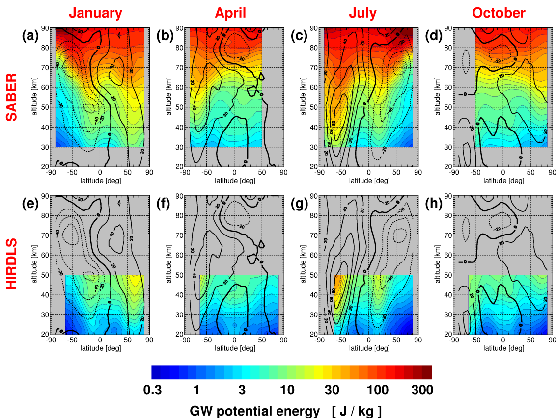
Figure 6. Latitude-altitude cross sections of gravity wave potential energies calculated after Eq. (3) from gravity wave temperature variances obtained directly after background removal. SABER variances are shown in the upper row, and HIRDLS variances in the lower row. Values are for average January (left column), April (second column), July (third column), and October (right column). Overplotted winds are from the SPARC climatology (Swinbank and Ortland, 2003; Randel et al., 2002, 2004). Westward (eastward) winds are indicated by dashed (solid) contour lines. The zero wind line is bold solid. Contour line increment is 20 \text{ m s}^{-1} .
