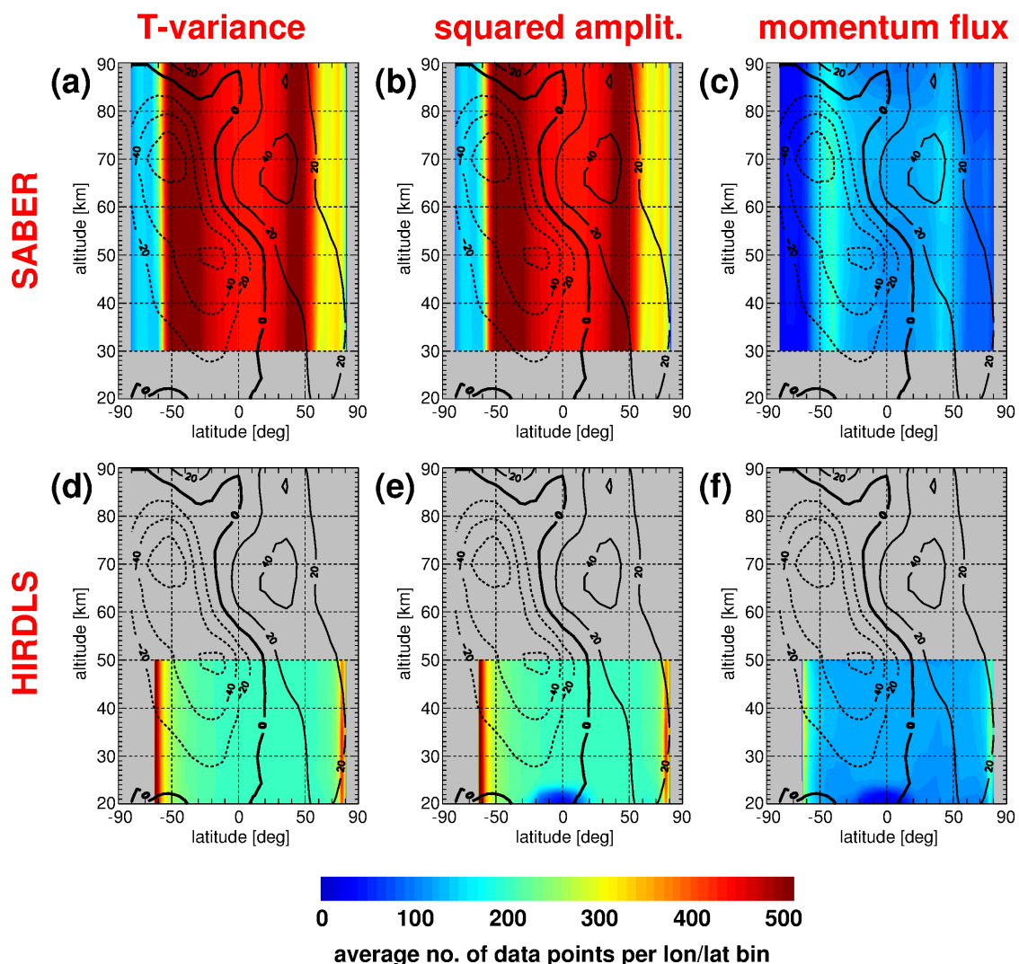
Figure 15. Latitude-altitude cross sections of the number of values per lon/lat bin used for global maps, zonally averaged for the average month of January. Shown are multi-year averages for SABER (upper) and HIRDLS (lower) for average global maps of gravity wave temperature variances (left column), squared amplitudes (center column), and absolute momentum fluxes (right column). Overplotted winds are from the SPARC climatology (Swinbank and Orland, 2003; Randel et al., 2002, 2004). Westward (eastward) winds are indicated by dashed (solid) contour lines. The zero wind line is bold solid. Contour line increment is 20 \text{ m s}^{-1} .
