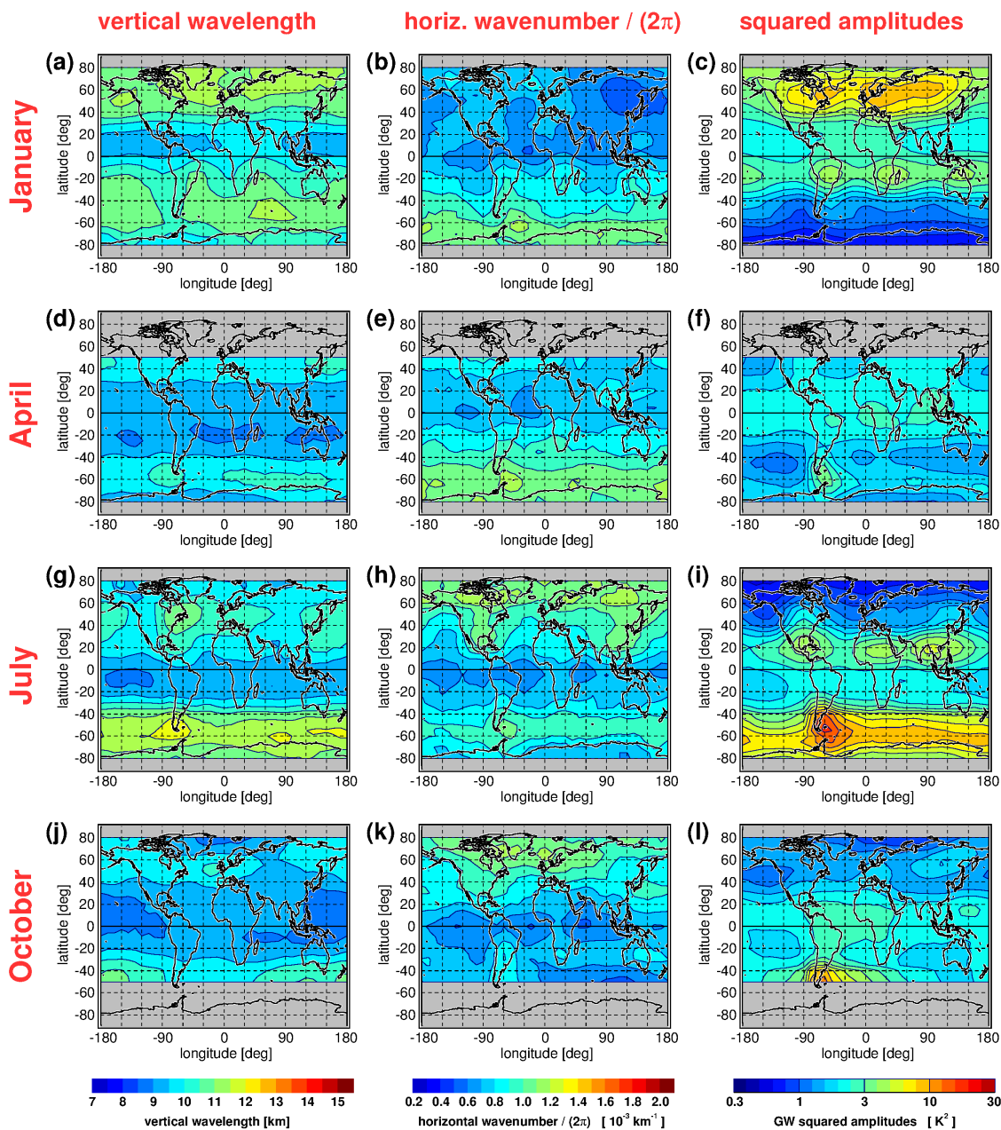
Figure 16. Global distributions of SABER 13-year average gravity wave vertical wavelengths (left column), horizontal wavenumbers k_h/(2\pi) (middle column), and squared amplitudes (right column) for different calendar months at 30 km altitude.
