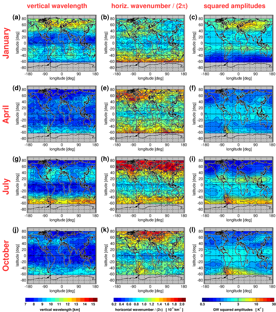
Figure 17. Global distributions of HIRDLS 3-year average gravity wave vertical wavelengths (left column), horizontal wavenumbers k_h/(2\pi) (middle column), and squared amplitudes (right column) for different calendar months at 30 km altitude.
