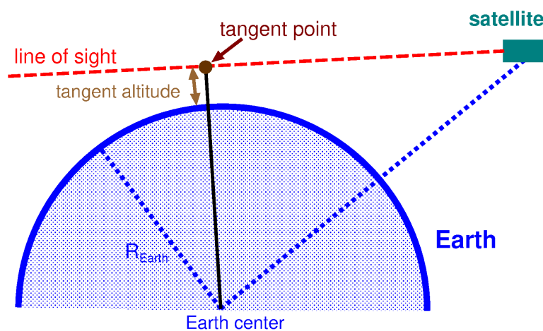
Figure 1. Schematic of the geometry of satellite limb observations. The satellite instrument views toward the Earth's horizon. The point of the instruments line of sight closest to the Earth surface is called tangent point, and the corresponding altitude is the tangent altitude.
