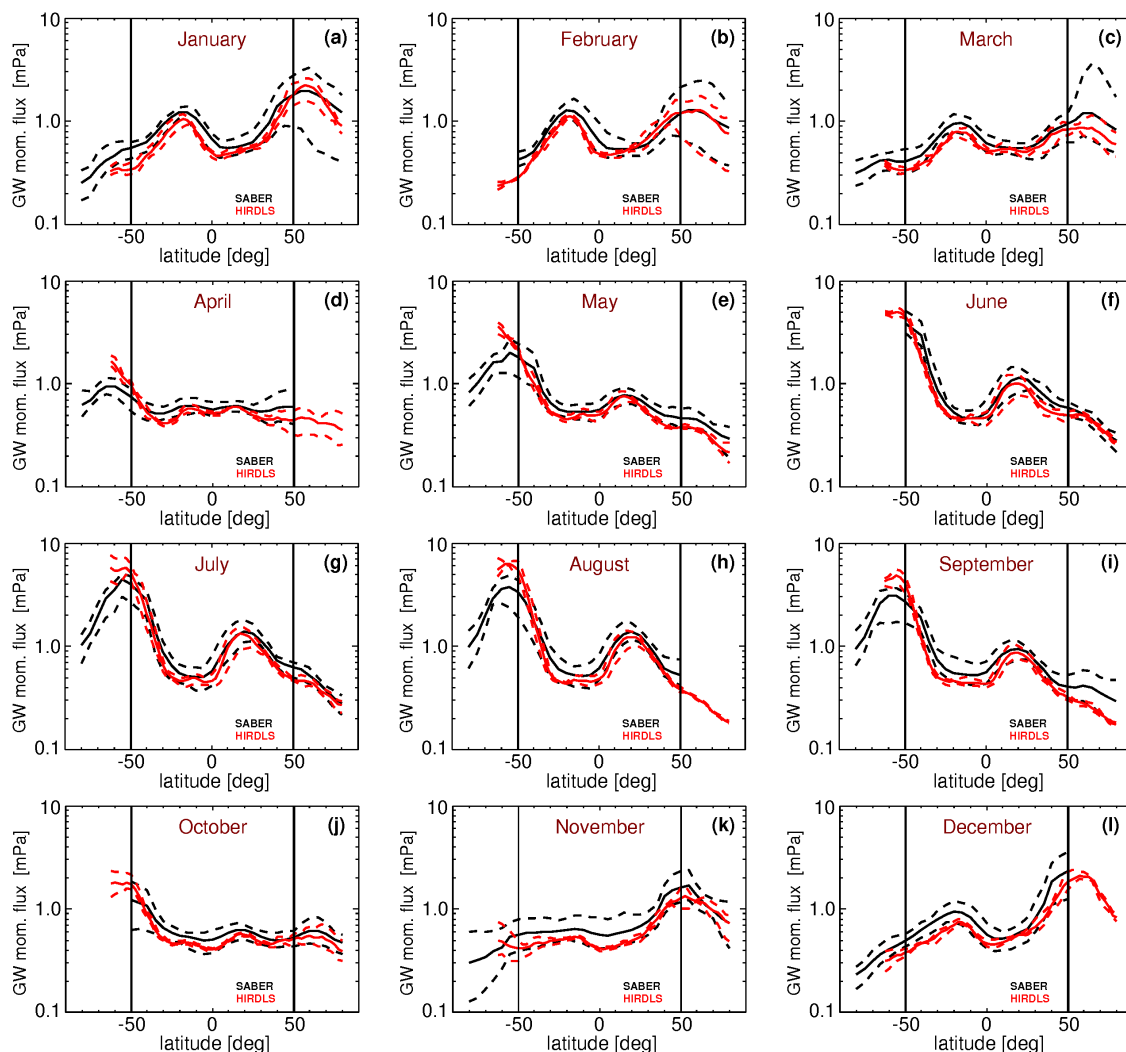
Figure 18. Zonal average gravity wave momentum fluxes at 30 km altitude. Shown are climatological averages for each calendar month (solid lines), as well as maximum and minimum values during the respective time period considered (dashed lines). SABER values are in black, and HIRDLS values are in red. The climatological averages are 13-year averages for SABER, and 3-year averages for HIRDLS, separately for each calendar month. Vertical lines at 50°S and 50°N indicate that only latitudes equatorward of 50° are continuously covered by SABER.
