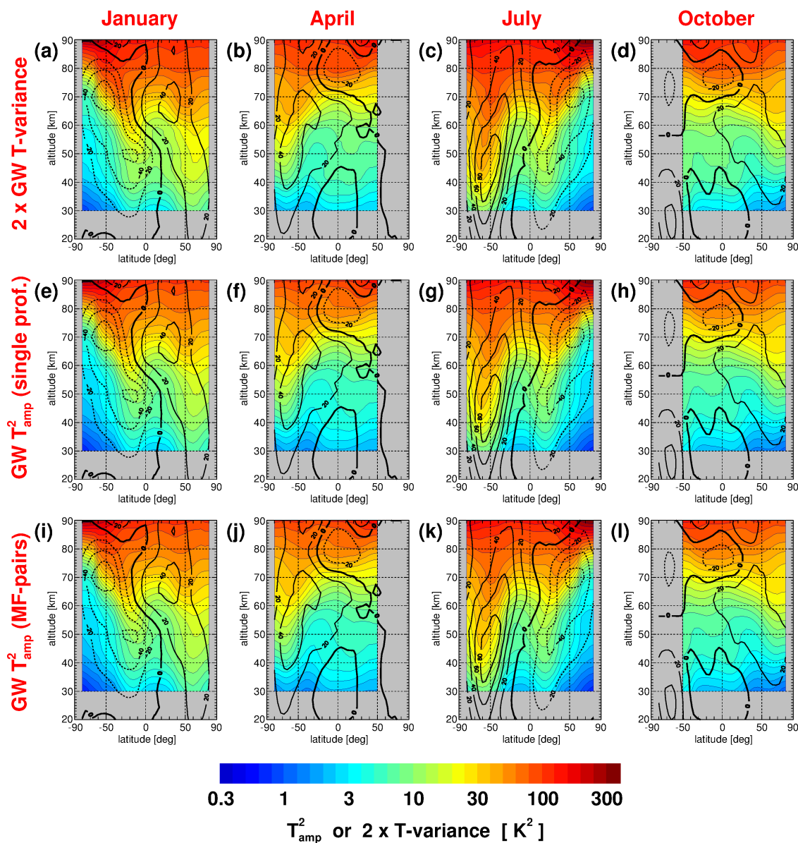
Figure 4. Latitude-altitude cross sections of SABER zonal average gravity wave temperature variances times 2 (upper), gravity wave squared amplitudes of single altitude profiles (middle), gravity wave squared amplitudes of pairs of altitude profiles utilized for determination of absolute momentum fluxes (lower). Values are for average January (left column), April (second column), July (third column), and October (right column). Overplotted winds are from the SPARC climatology (Swinbank and Orland, 2003; Randel et al., 2002, 2004). Westward (eastward) winds are indicated by dashed (solid) contour lines. The zero wind line is bold solid. Contour line increment is 20 \text{ m s}^{-1} .
