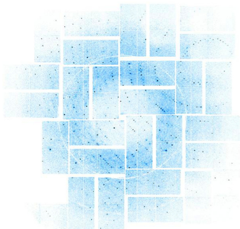
Figure 54: Diffraction image from a single nanocrystal built from the protein lysozyme [AHC14]. The distribution of the rectangles corresponds to the location of the sub-panel within the front panel at the LCLS. The dark spots show the Bragg-spots. The photon background is given by the “halo ring” around the beamhole at the centre of the detector.
