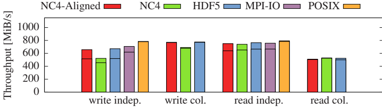
Figure 47: Performance with disjoint pattern.
