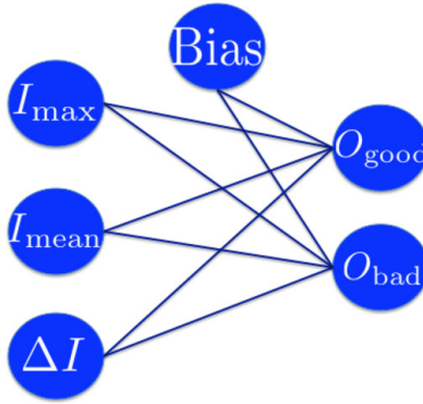
Figure 57: Neural network with three input neurons, two output neurons and no hidden layer.
