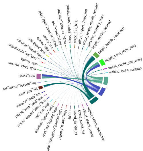
Figure 52: Visualization of latent paths from hidden to emitting states of Lustre logging data.
