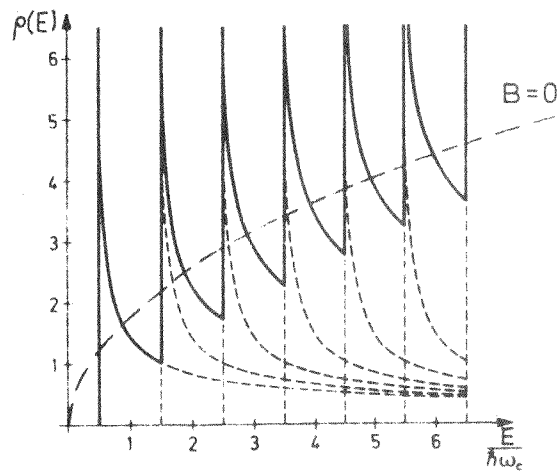
Fig. 2.3 The density of states for free electrons in an applied magnetic field. (Dashed lines show contributions from individual Landau cylinders, long dashes show the density of states in the absence of a field.)
