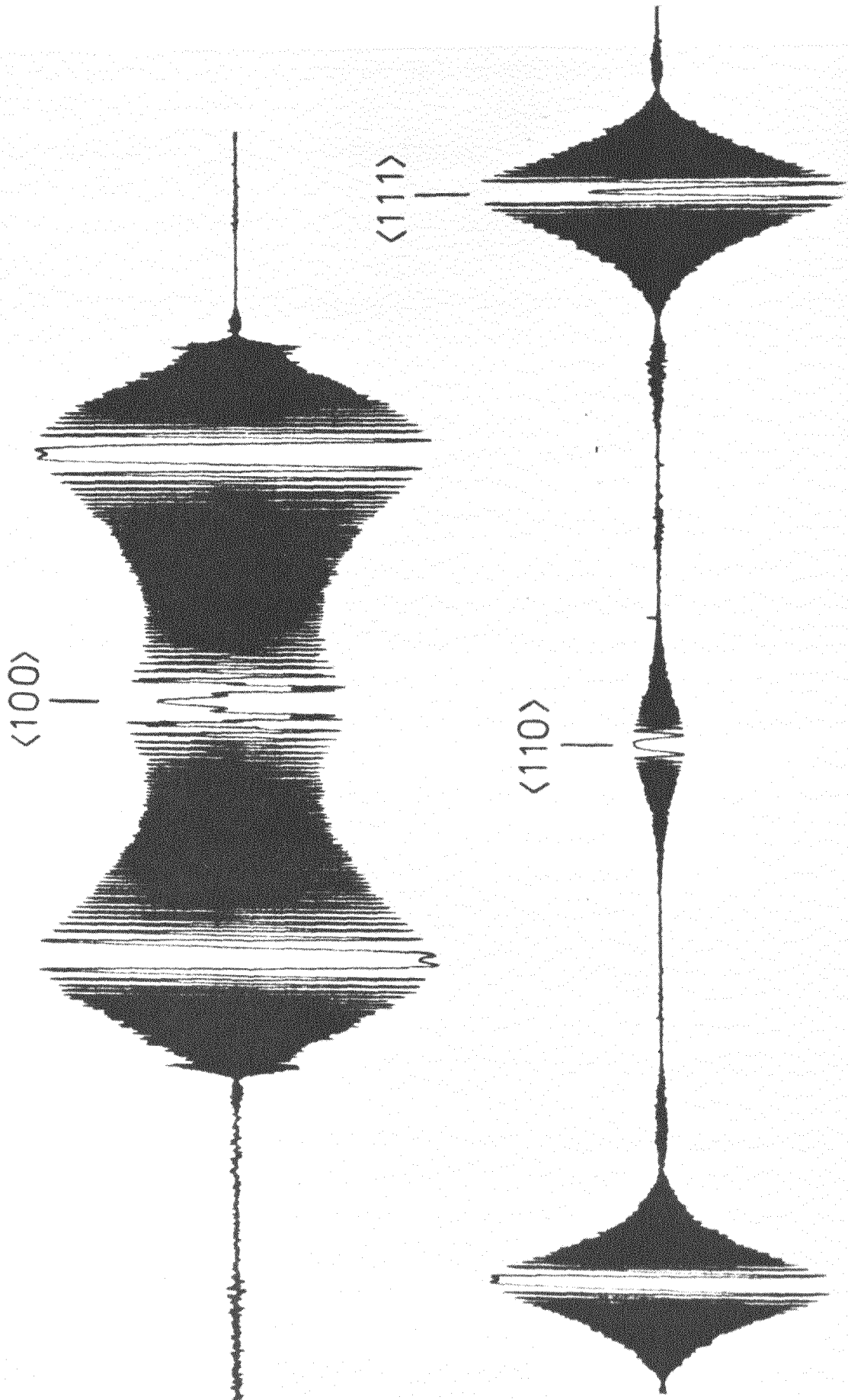
Fig. 3.7 Recording of dHvA signal versus orientation of a Cu sample in the magnetic field in a plane (110).
