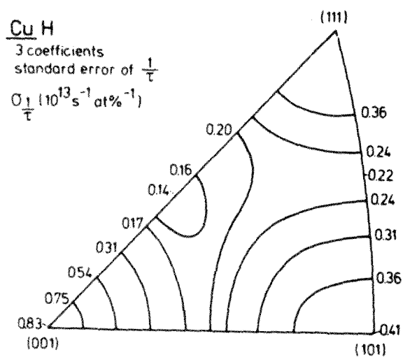
Fig. A1 Contour plots of the local scattering rate 1/\tau(\underline{k}) for Cu-H over the basic 1/48 th of the Fermi surface in stereographic projection. Shown are the scattering rates from the three and four coefficient fits as discussed in the text and the standard error in 1/\tau(\underline{k}) for the three coefficient fit.
