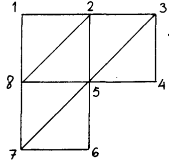
Fig.3 (3-node elements)
