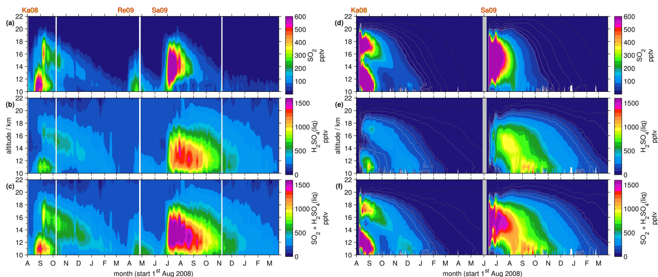
Figure 7. \text{SO}_2 , liquid-phase \text{H}_2\text{SO}_4 , and total sulphur ( \text{SO}_2 + \text{H}_2\text{SO}_4 ) volume mixing ratios by MIPAS (a–c) and the CTM (d–f). Vertically resolved time series of \text{SO}_2 and sulphate aerosol for 30^\circ \text{N} – 90^\circ \text{N} , starting on the 1 Aug 2008 (area weighted 5d running means). Indicated are the days of the eruptions of the volcanoes Kasatochi in Aug 2008, Redoubt in Mar 2009, and Sarychev in Jun 2009. The colour scale is restricted to 0–800 pptv ( \text{SO}_2 ), and 0–1,600 pptv (sulphate aerosol, and sum of \text{SO}_2 and sulphate aerosol). Lower and higher values are assigned with the respective limiting value. For the CTM contour lines in dark to light grey represent 1, 5, 10, 20, 30, and 40 pptv in the case of \text{SO}_2 , and 5, 25, 50, 100, 150, and 200 pptv for sulphate aerosol, and the sum of \text{SO}_2 and sulphate aerosol. For the CTM two simulations are shown, from August 2008 to May 2009, and from June 2009 to May 2010, separated by a bold grey line.
