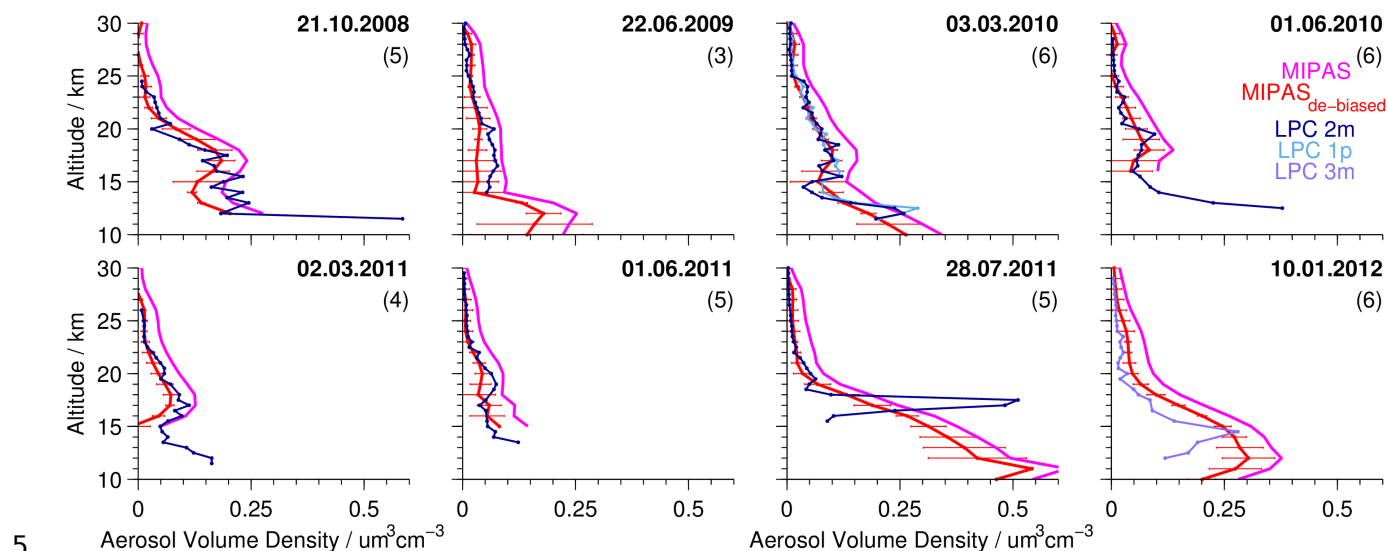
Figure 3. Profiles of aerosol volume densities from in situ and MIPAS satellite measurements. In situ data are balloon-borne data above the lapse rate tropopause for Laramie, Wyoming ( 41^\circ \text{N}/105^\circ \text{W} ), measured by Laser Particle Counters (LPCs). MIPAS satellite data in pink (original data) and red (de-biased data). For all MIPAS data the ice filter by Griessbach et al. (2016) and ash filter by Griessbach et al. (2014) are applied. MIPAS profiles are averages of all available profiles for the indicated day, averaged in a \pm 5^\circ \text{lat} \times 10^\circ \text{lon} area. In brackets are the number of MIPAS profiles included in the average. For the de-biased MIPAS values the standard deviations of the mean profiles are shown.
