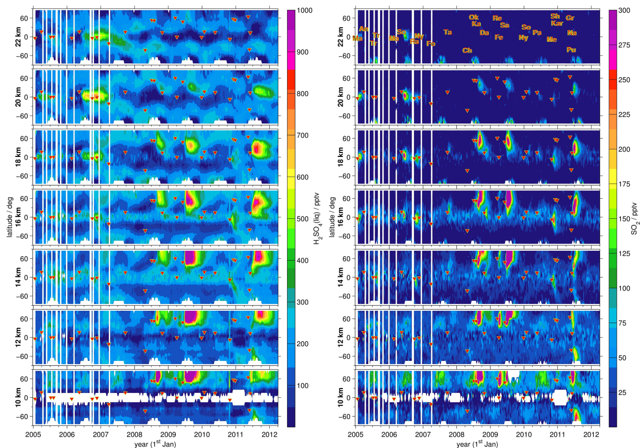
Figure 5. Global time series of latitudinally resolved distributions of MIPAS liquid-phase \text{H}_2\text{SO}_4 (left panels) and \text{SO}_2 (right panels) volume mixing ratios. Shown are 8-day mean values for 10^\circ latitude bins at different altitudes (10 to 22 km). The colour code is restricted to 0–1,000 pptv for \text{H}_2\text{SO}_4(\text{liq}) , and 0–300 pptv for \text{SO}_2 . Values exceeding these limits are assigned with the limiting value, respectively. Volcanic eruptions are indicated by red triangles (together with their abbreviated names in the uppermost right panel; from Höpfner et al., 2015; Table 3 therein).
