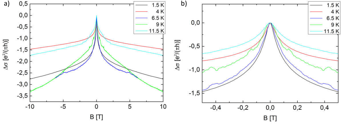
Fig. 7.10: WAL curves for different temperatures. b) shows the range from -0.5 T to 0.5 T of a), which is also the range to which the HLN equation is fitted.
