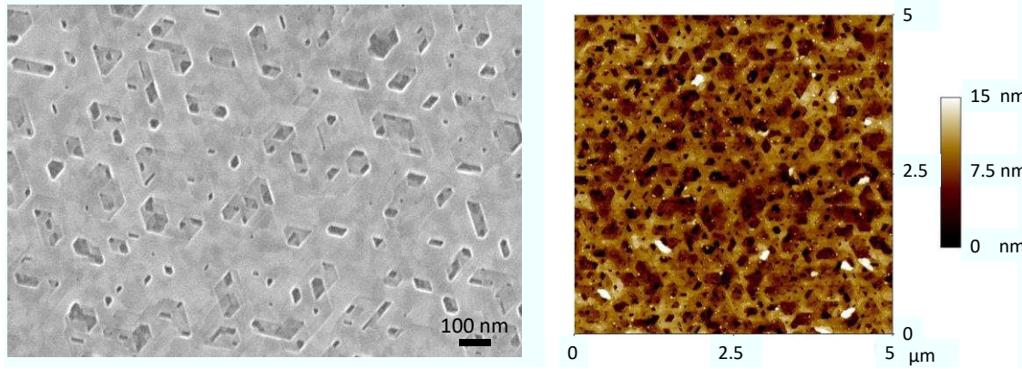
Fig. 4.8: SEM image of \text{Bi}_2\text{Se}_3 grown on \text{InP:Fe} with the same growth parameters as in Fig. 4.7, but with an additional annealing step after growth, in this case 20 min at 330 °C. On the right, an atomic force microscope picture of the \text{Bi}_2\text{Se}_3 film surface is shown. The colorbar is fixed to the highest measured value.
