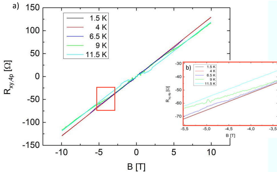
Fig. 7.8: Graph a) shows the Hall resistance R_{xy,4p} at different temperatures from 1.5 K to 11.5 K in steps of 2.5 K. b) shows the highlighted area of figure a).
