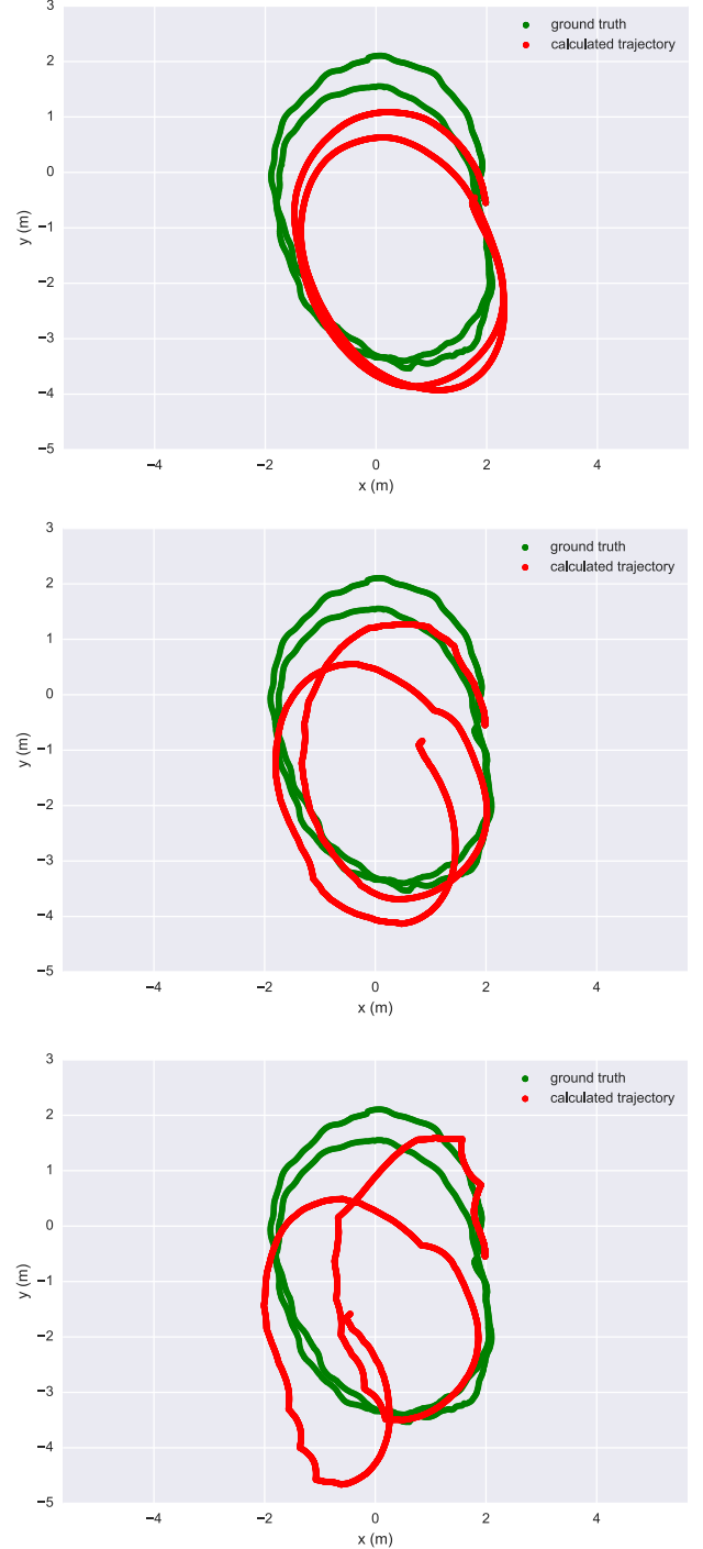
Fig. 3. Calculated IMU trajectory and ground truth trajectory of the evacuation chair for v_{range} = 0.01 (top), v_{range} = 0.05 (middle) and v_{range} = 0.10 (bottom).
