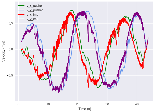
Fig. 4. Velocity of the evacuation chair (ground truth) and corrected velocity based on data of the IMU and pushing person.
